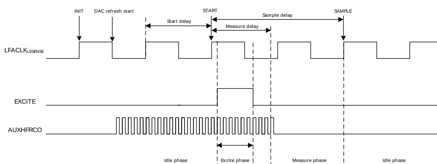
Figure 21.3. Timing diagram, short excitation
