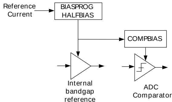
Figure 24.5. ADC Bias Programming
