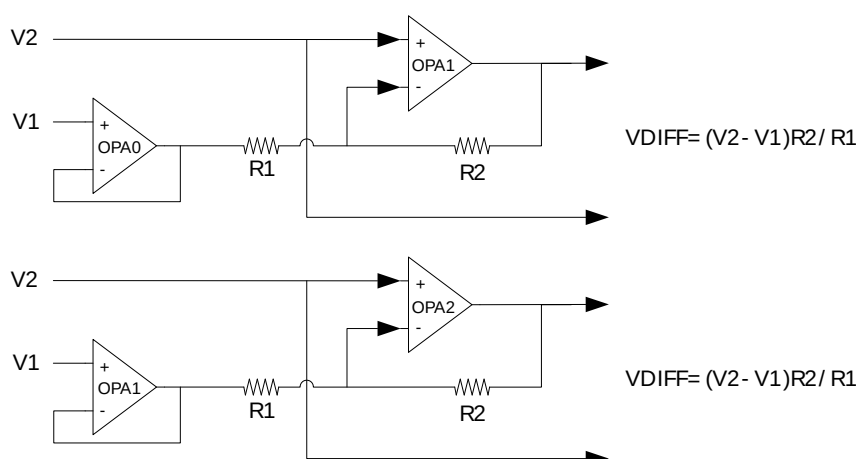
Figure 26.9. Two Op-amp Differential Amplifier Overview
