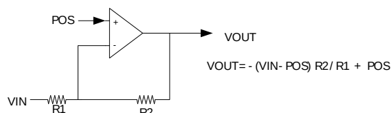
Figure 26.5. Inverting input PGA Overview
