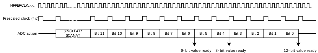
Figure 24.2. ADC Conversion Timing
