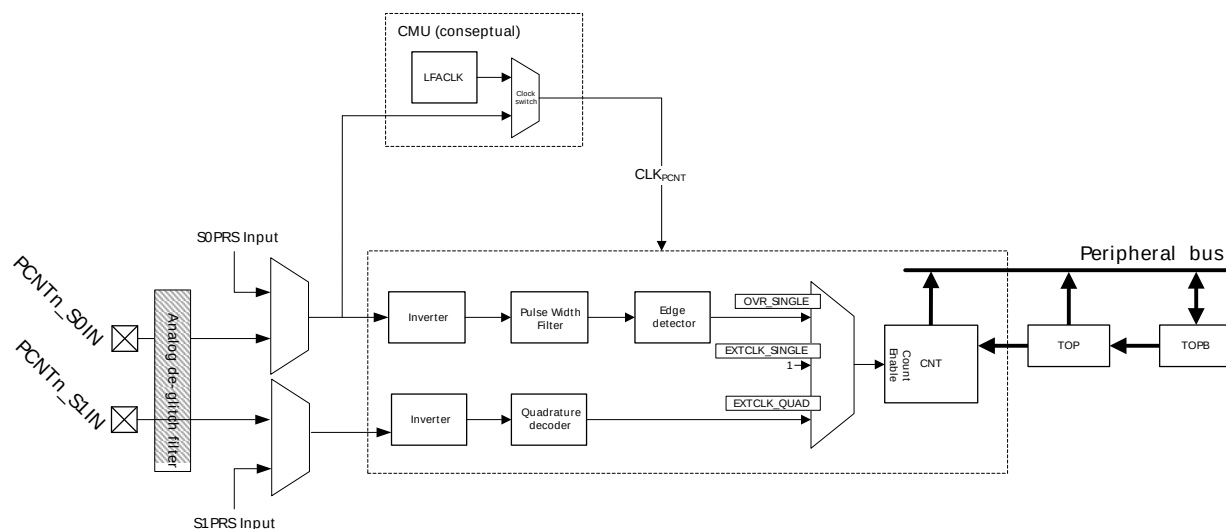
Figure 20.1. PCNT Overview
