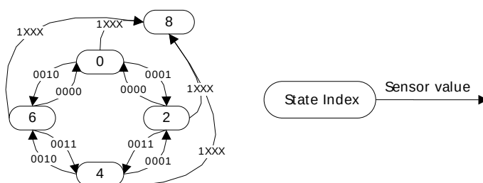
Figure 21.14. FSM example 2
