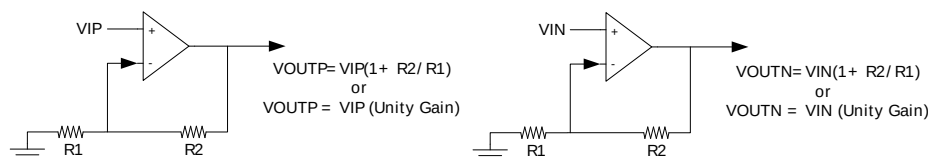
Figure 26.11. Dual Buffer ADC Driver Overview
