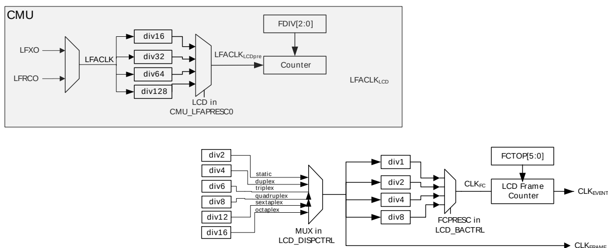
Figure 29.43. LCD Clock System in LCD Driver
