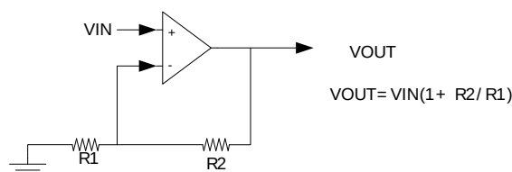
Figure 26.6. Non-inverting PGA Overview
