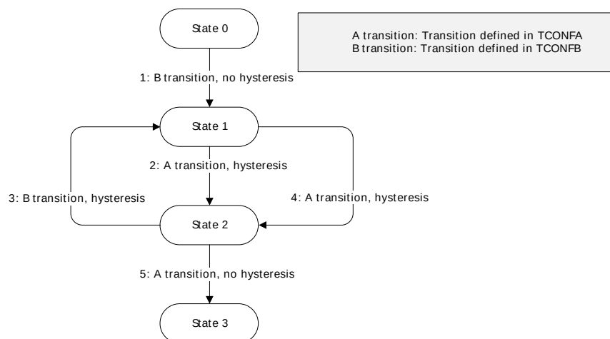
Figure 21.8. Decoder hysteresis
