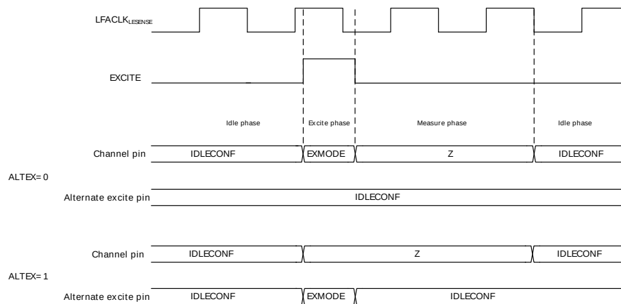
Figure 21.4. Pin sequencing
