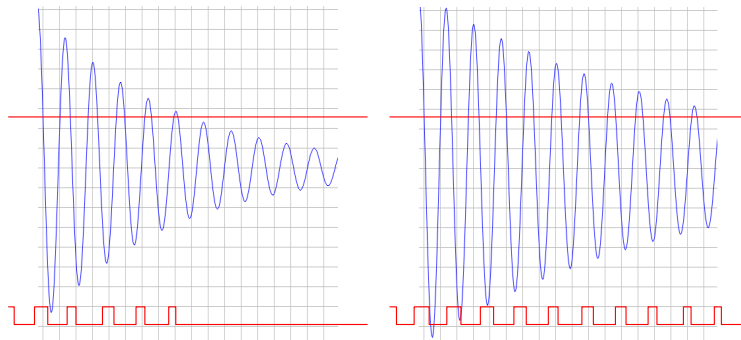
Figure 21.12. LC sensor oscillations
