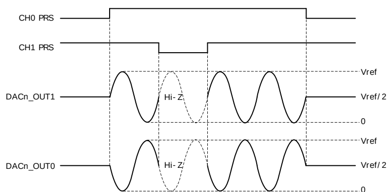
Figure 25.3. DAC Sine Mode
