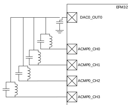
Figure 21.11. LC sensor setup
