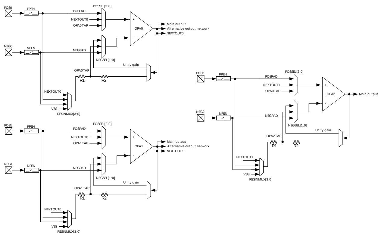
Figure 26.2. OPAMP Overview
