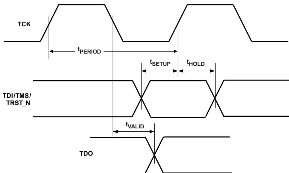
Figure 4-21. JTAG Timing
