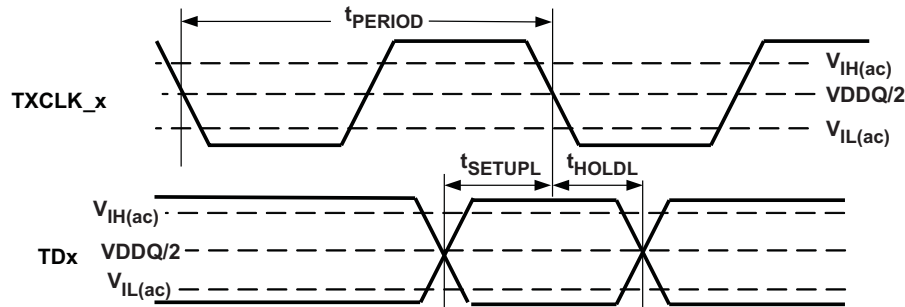
Figure 4-19. HSTL (SDR Timing Mode Only) Rising Edge Aligned (Falling Edge Sampled) Data Input Timing Requirements
