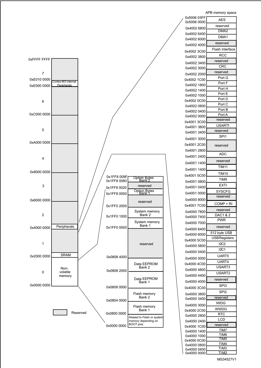
Figure 7. Memory map
