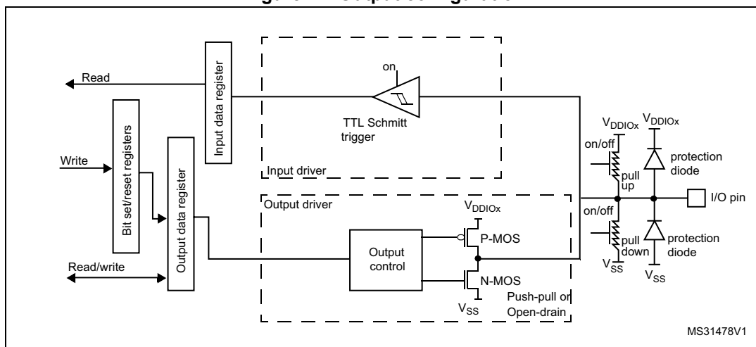
Figure 24. Output configuration
