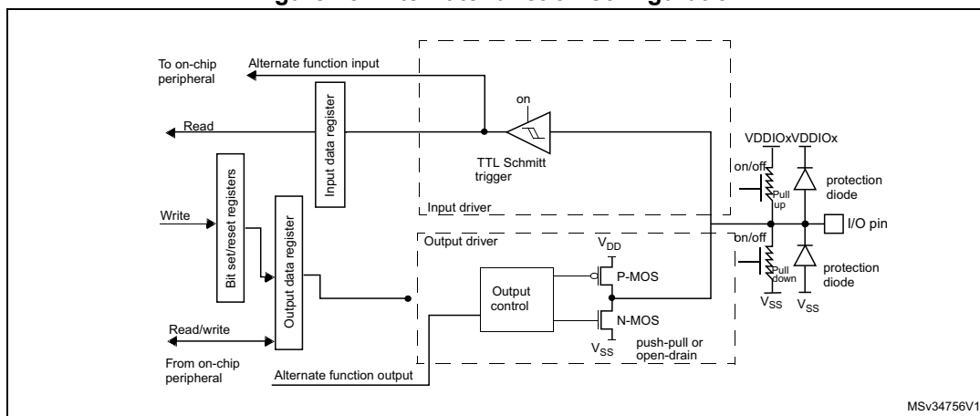
Figure 25. Alternate function configuration
