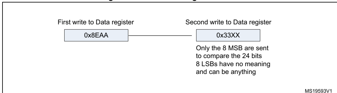
Figure 280. Transmitting 0x8EAA33
