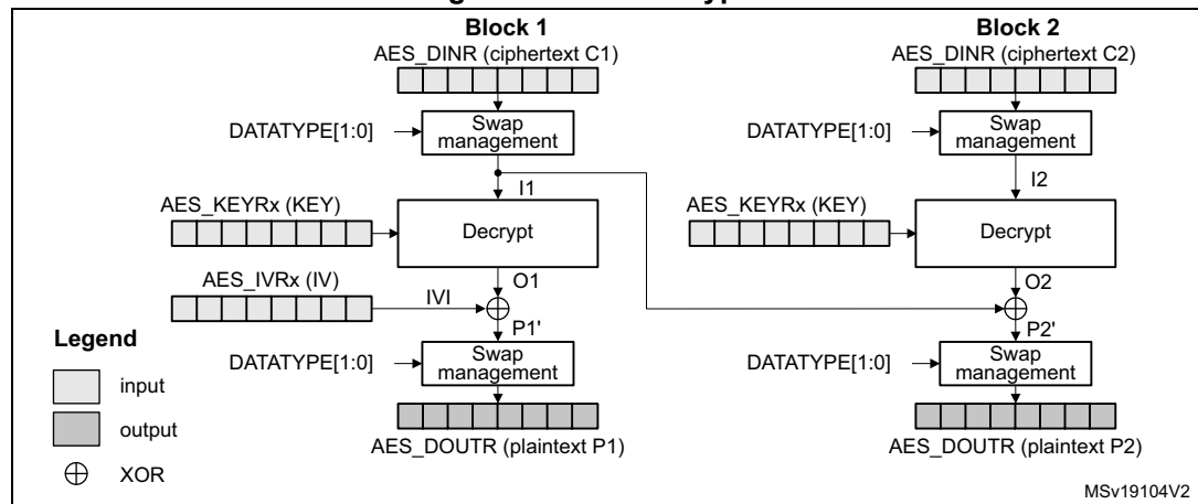
Figure 77. CBC decryption
