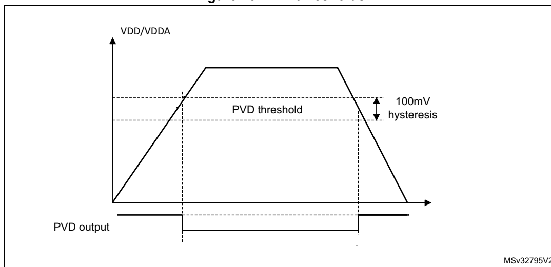
Figure 15. PVD thresholds
