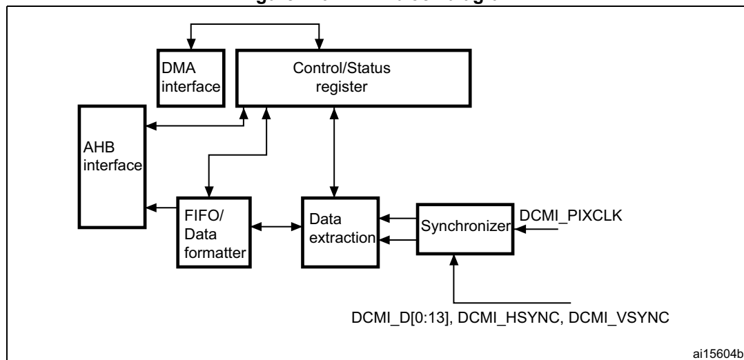
Figure 110. DCMI block diagram
