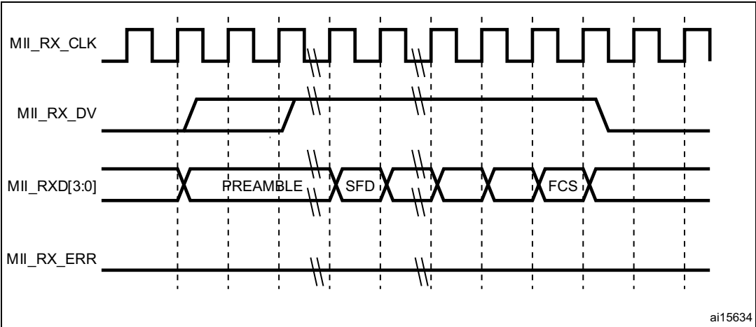
Figure 558. Reception with no error
