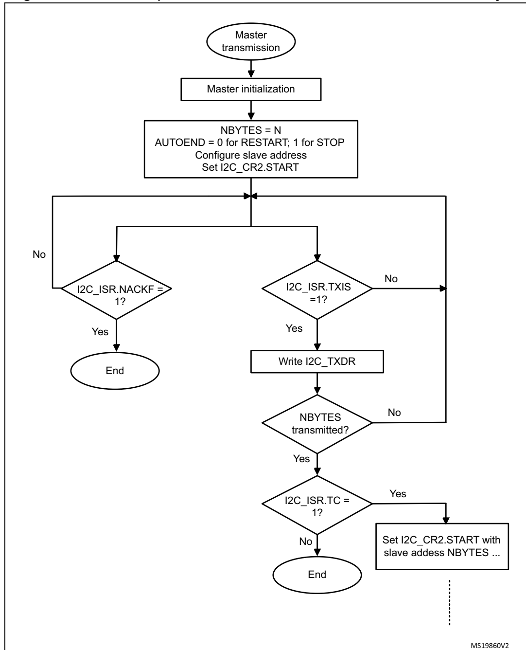
Figure 366. Transfer sequence flowchart for I2C master transmitter for N \leq 255 bytes
