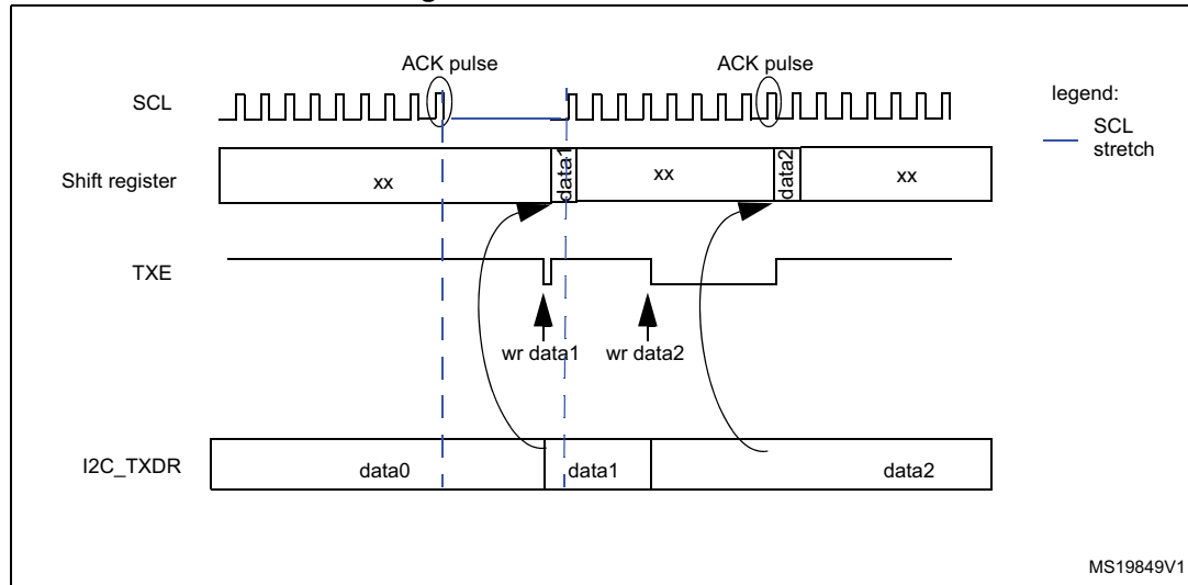
Figure 354. Data transmission
