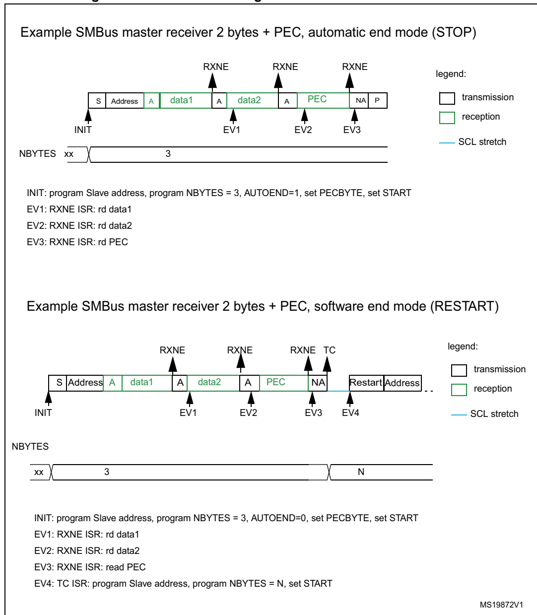
Figure 378. Bus transfer diagrams for SMBus master receiver
