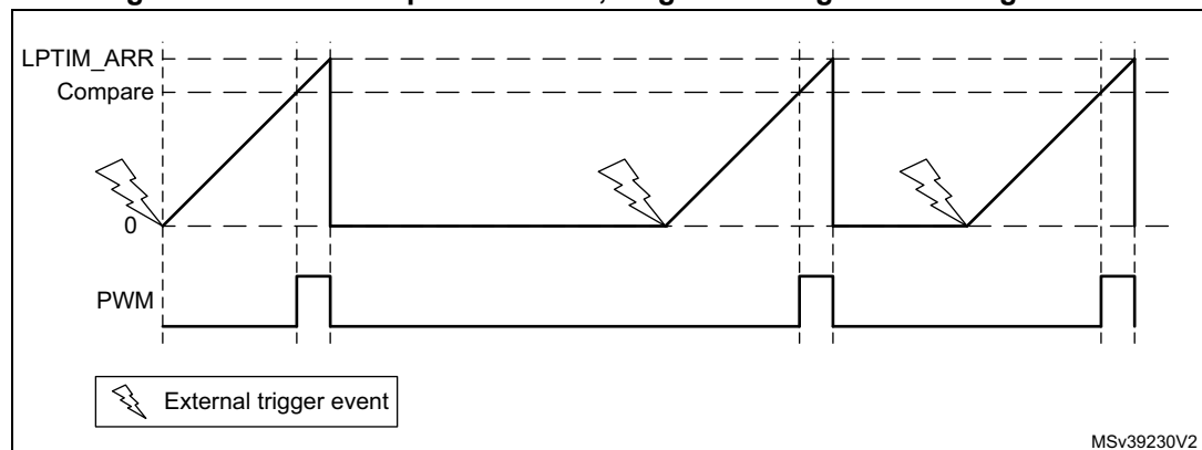
Figure 340. LPTIM output waveform, single counting mode configuration
