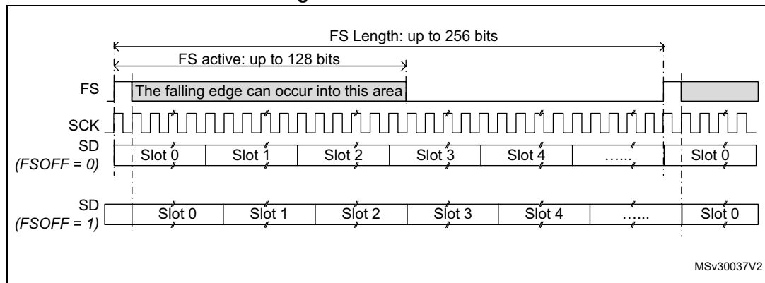
Figure 444. Audio frame
