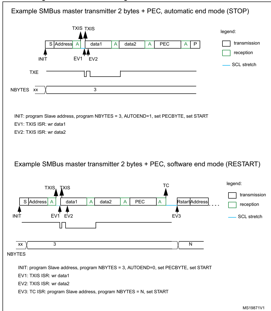
Figure 377. Bus transfer diagrams for SMBus master transmitter
