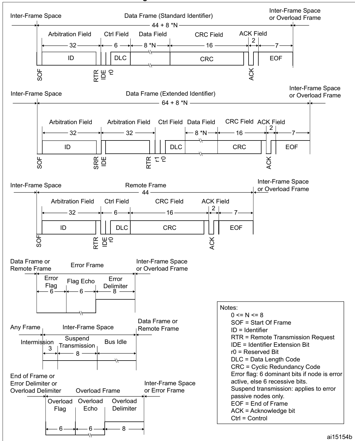
Figure 506. CAN frames
