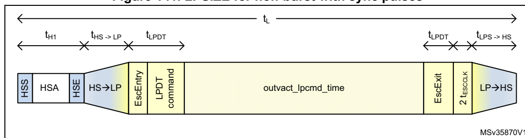
Figure 141. LPSIZE for non-burst with sync pulses
