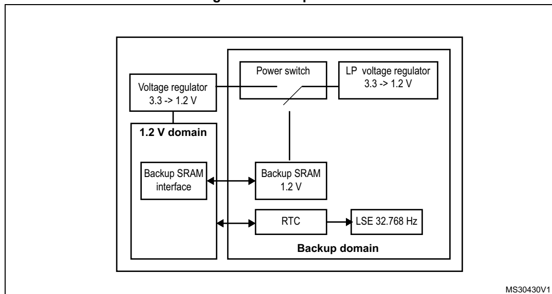
Figure 8. Backup domain
