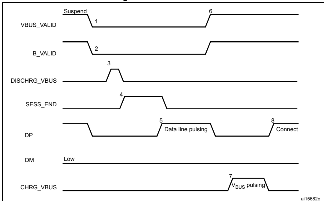
Figure 538. B-device SRP
