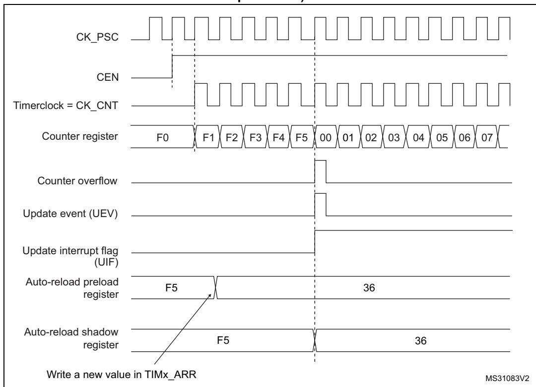
Figure 261. Counter timing diagram, Update event when ARPE=1 (TIMx_ARR preloaded)
