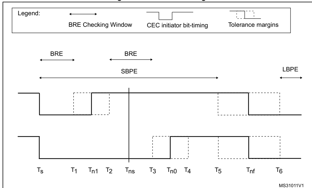
Figure 585. Error handling
