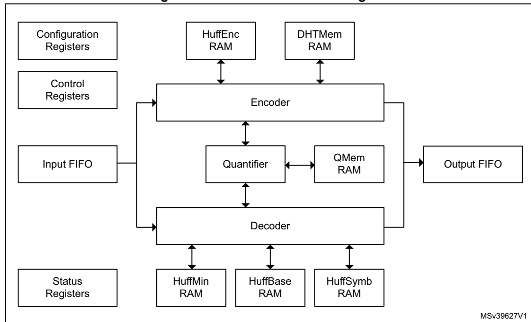
Figure 161. JPEG codec block diagram
