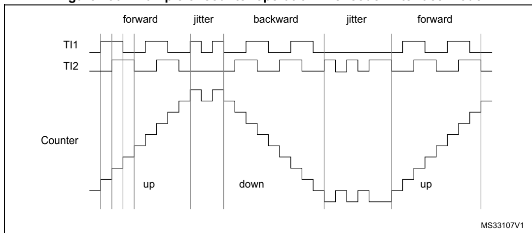
Figure 290. Example of counter operation in encoder interface mode
