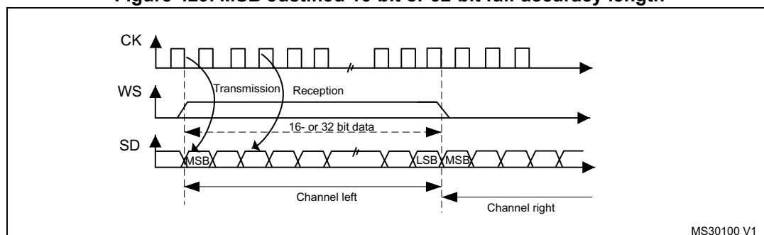
Figure 429. MSB Justified 16-bit or 32-bit full-accuracy length
