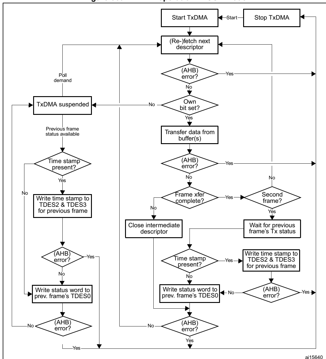
Figure 569. TxDMA operation in OSF mode
