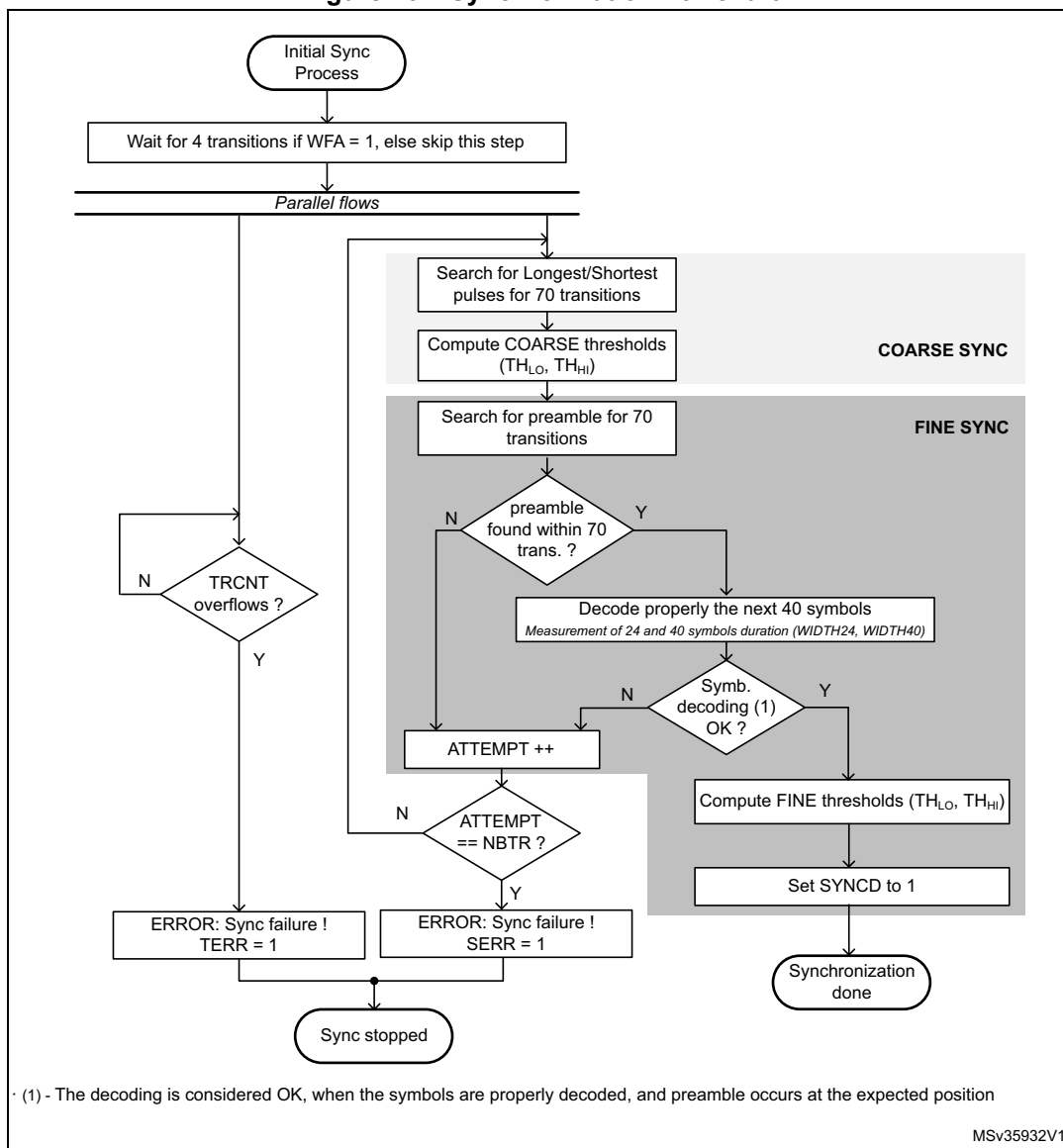
Figure 467. Synchronization flowchart
