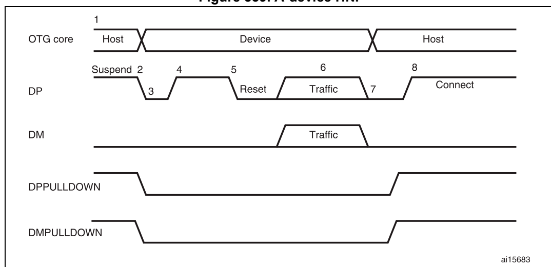
Figure 539. A-device HNP
