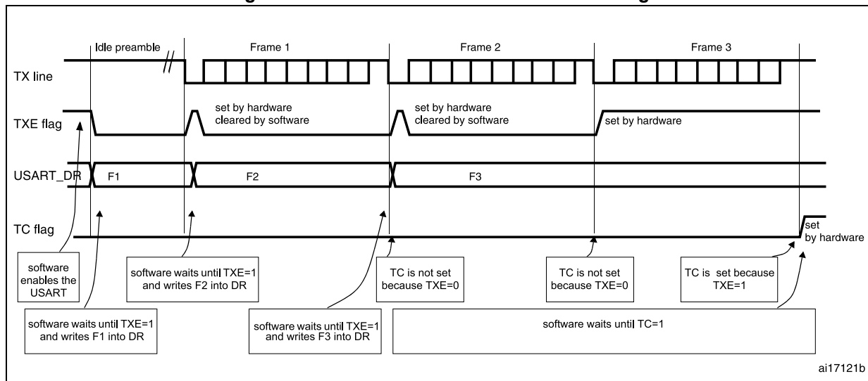
Figure 383. TC/TXE behavior when transmitting
