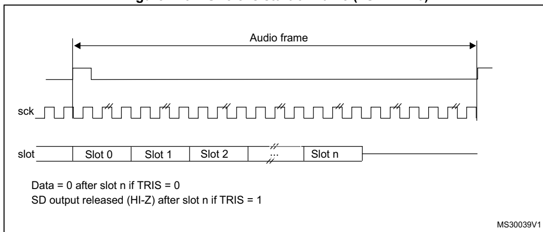
Figure 446. FS role is start of frame (FSDEF = 0)
