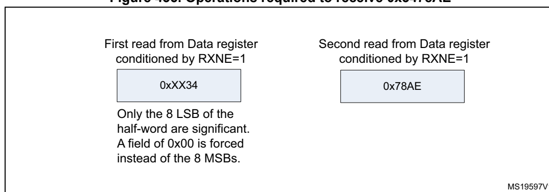
Figure 435. Operations required to receive 0x3478AE
