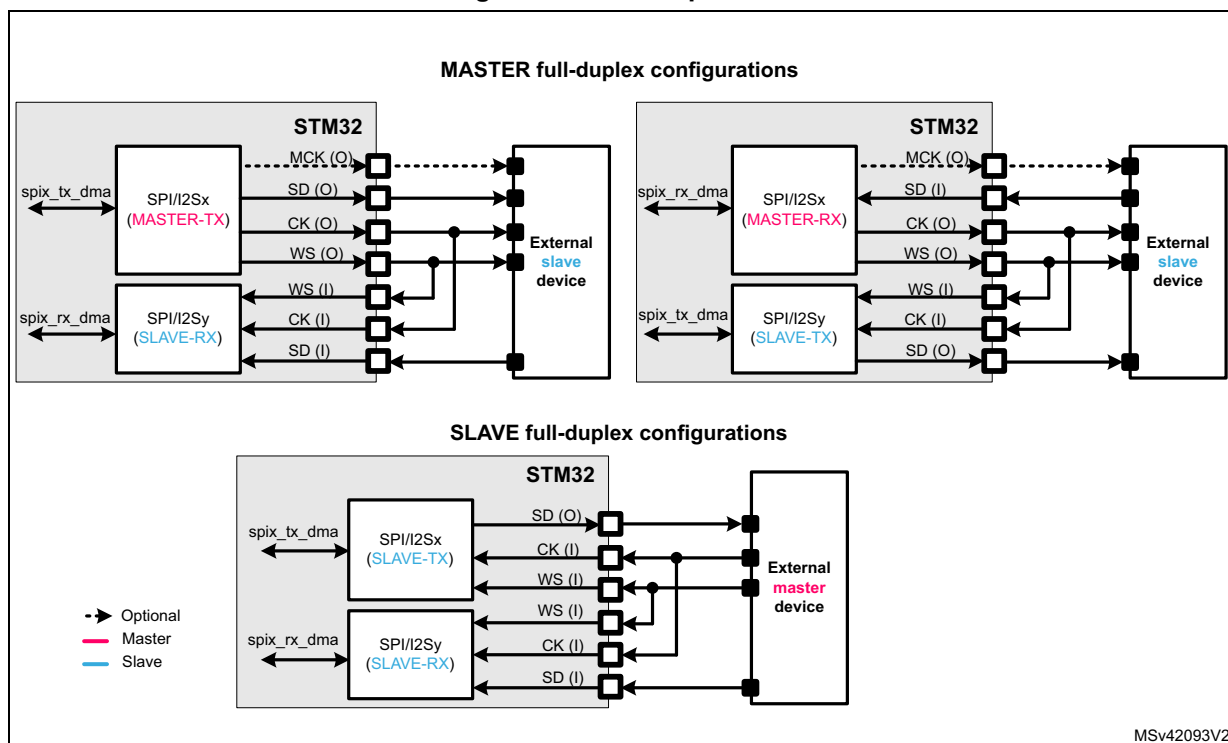
Figure 422. Full-duplex communication
