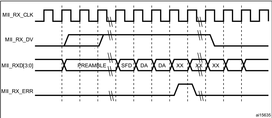
Figure 559. Reception with errors
