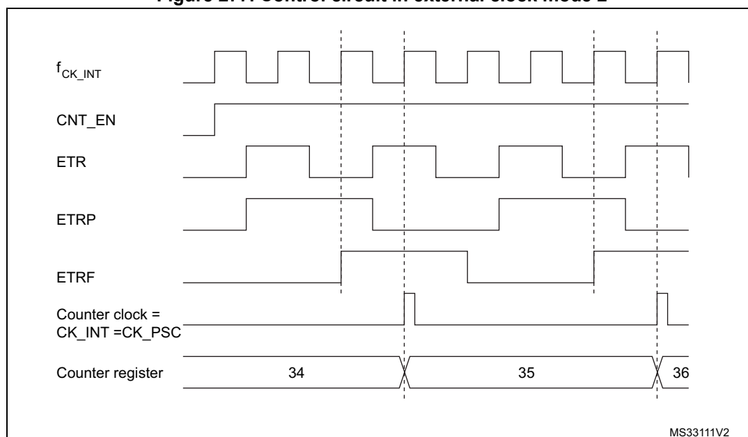
Figure 277. Control circuit in external clock mode 2
