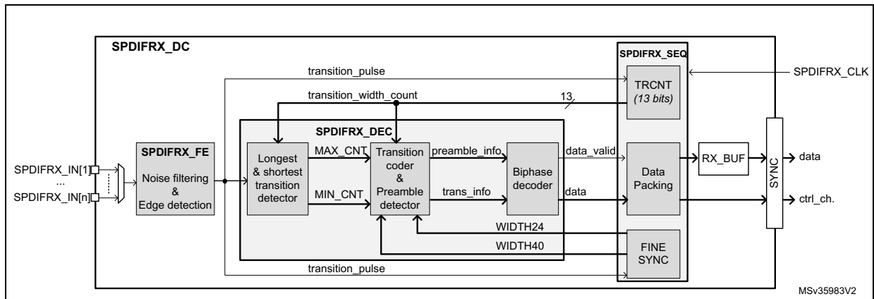
Figure 464. SPDIFRX decoder
