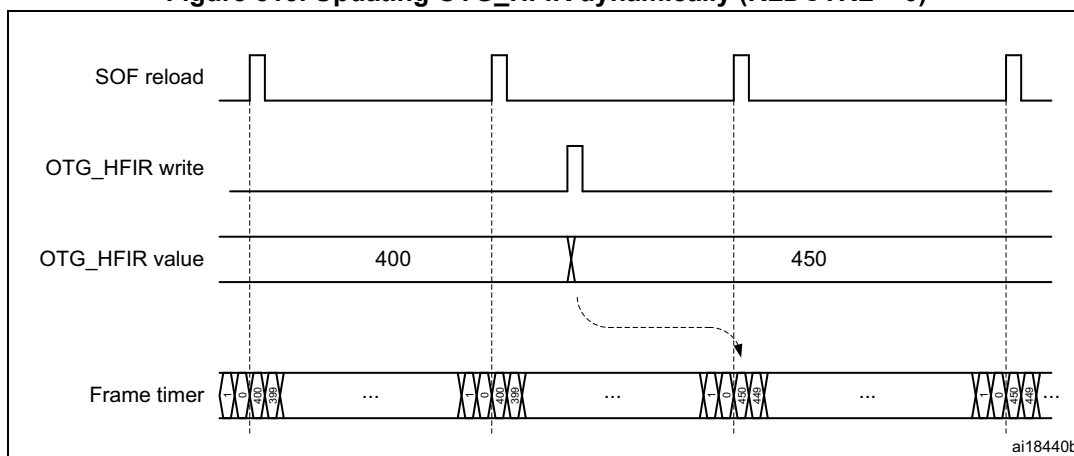
Figure 515. Updating OTG_HFIR dynamically (RLDCTRL = 0)
