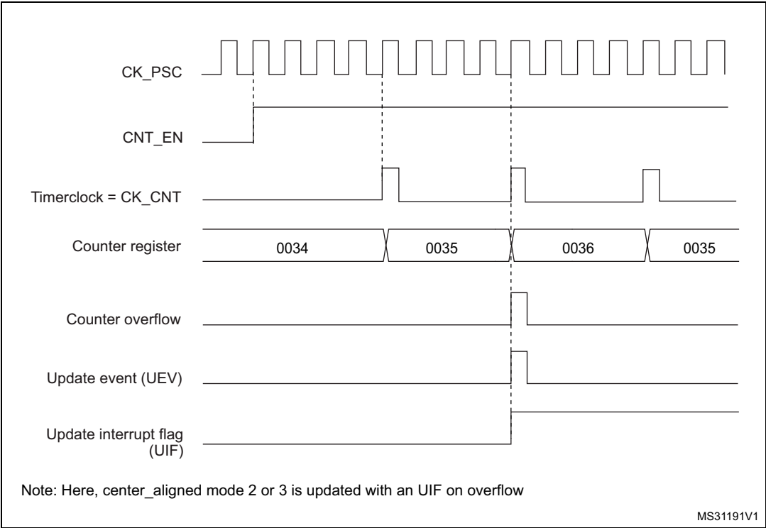
Figure 269. Counter timing diagram, internal clock divided by 4, TIMx_ARR=0x36
