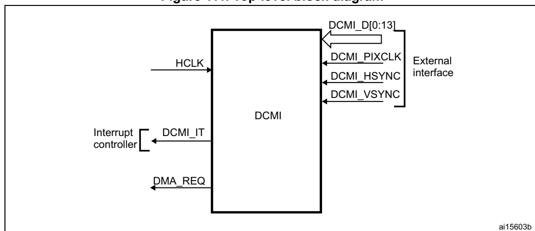
Figure 111. Top-level block diagram
