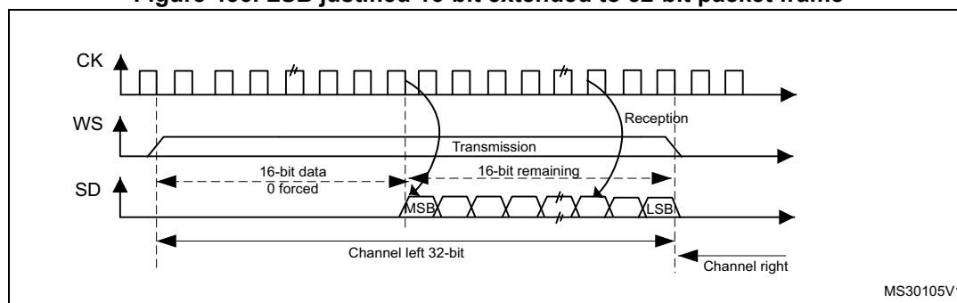
Figure 436. LSB justified 16-bit extended to 32-bit packet frame
