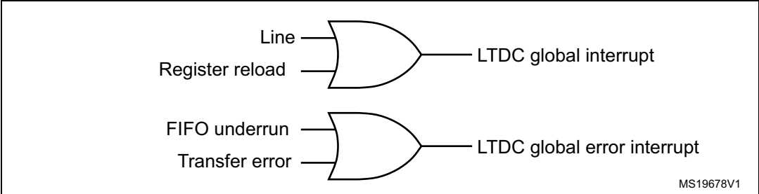
Figure 123. Interrupt events
