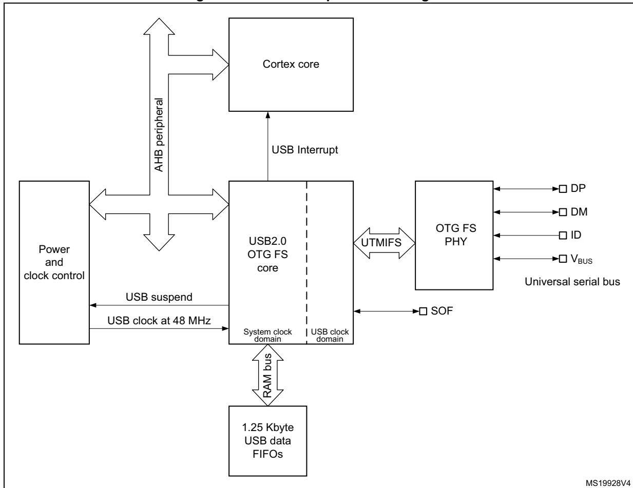
Figure 509. OTG full-speed block diagram
