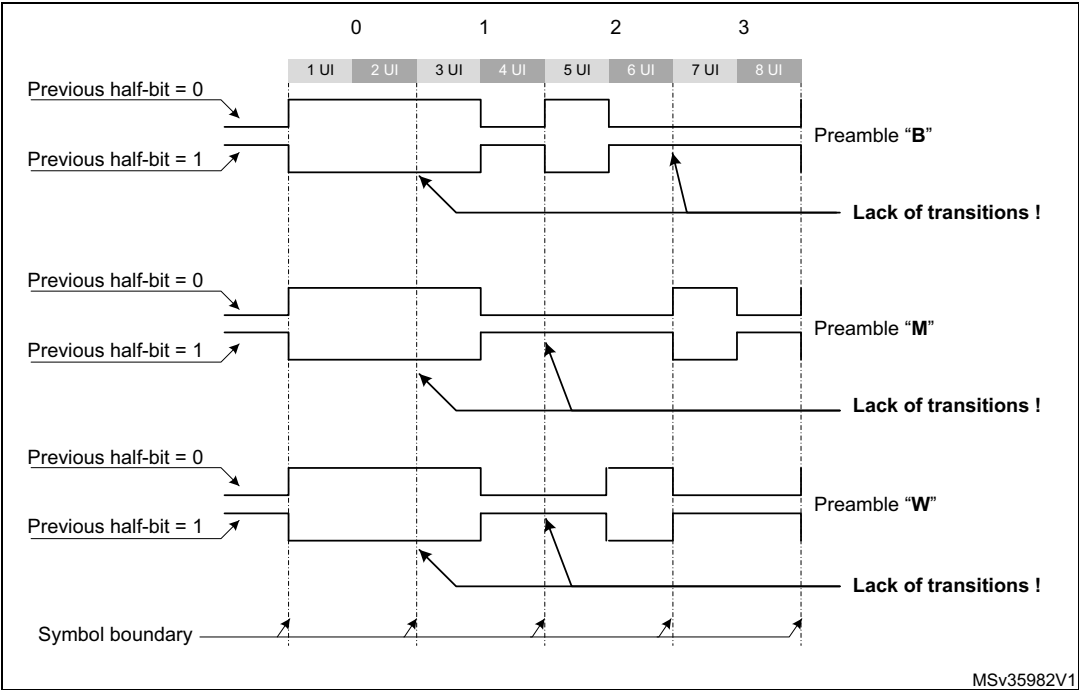
Figure 462. S/PDIF Preambles
