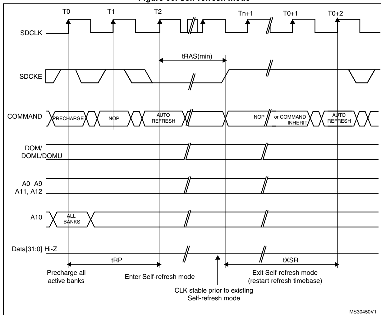
Figure 60. Self-refresh mode
