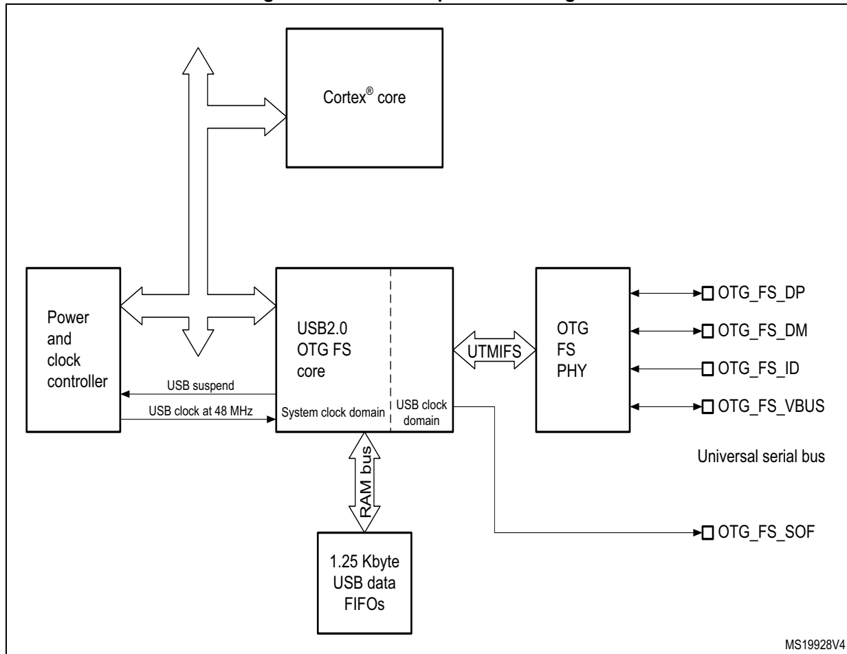
Figure 457. OTG full-speed block diagram
