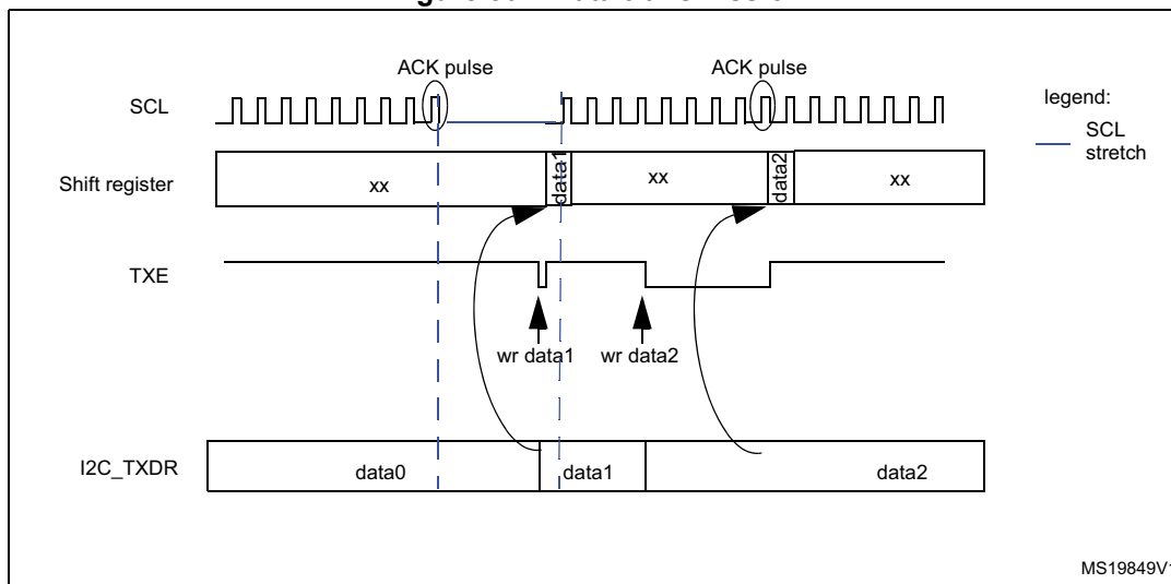
Figure 307. Data transmission
