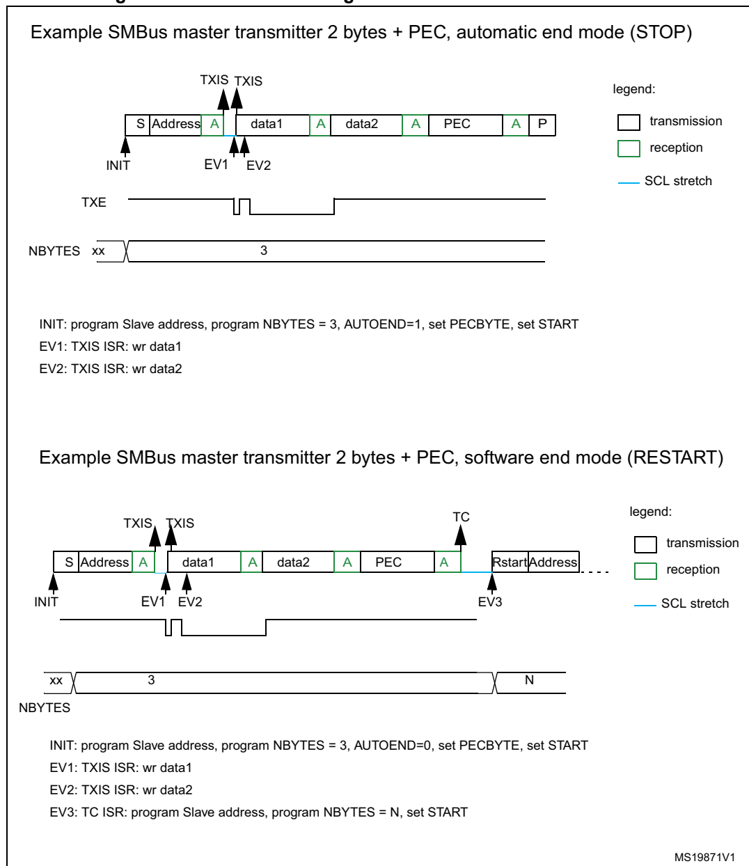
Figure 330. Bus transfer diagrams for SMBus master transmitter
