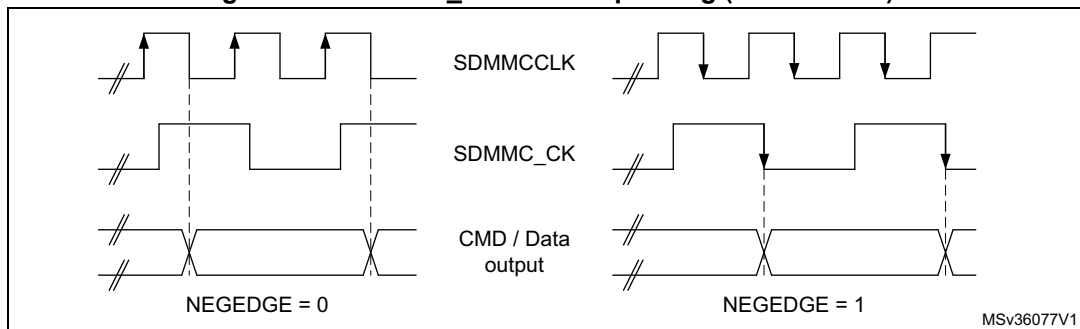
Figure 435. SDMMC_CLK clock dephasing (BYPASS = 0)
