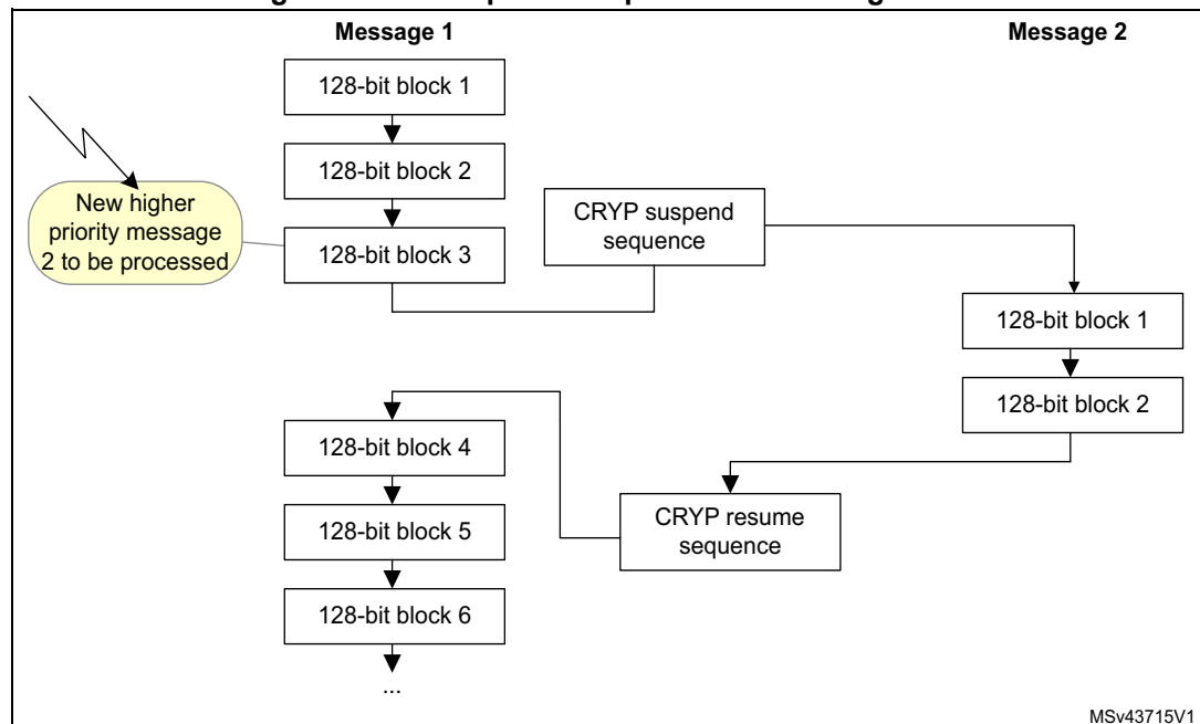
Figure 127. Example of suspend mode management
