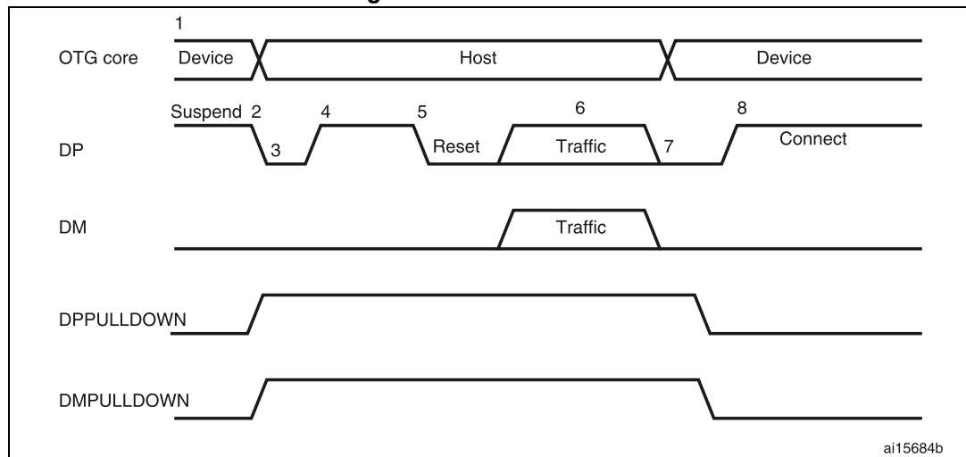
Figure 488. B-device HNP
