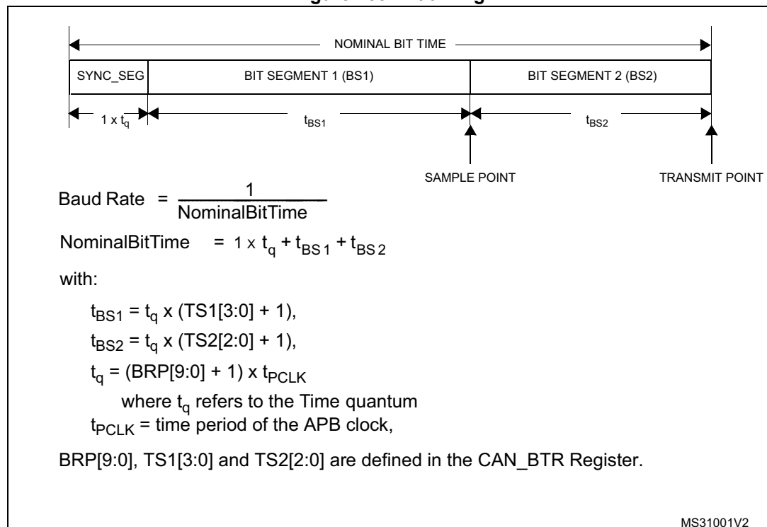
Figure 453. Bit timing
