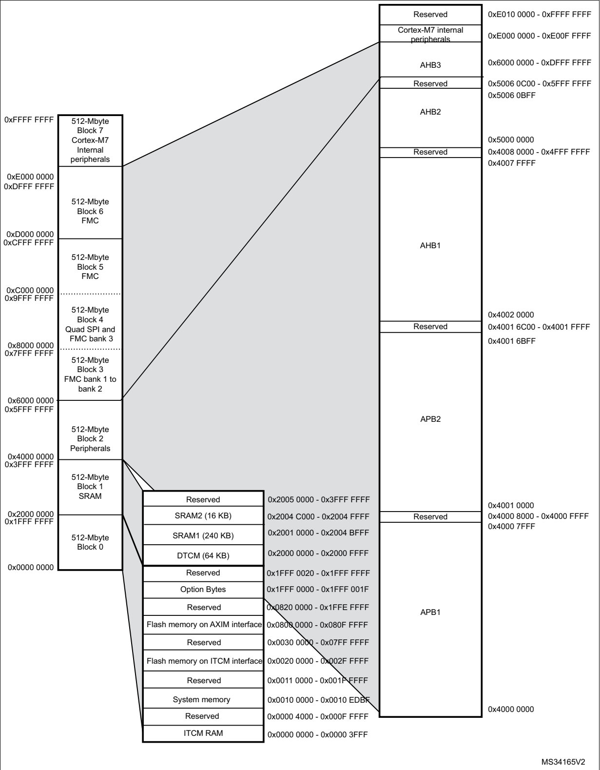
Figure 2. Memory map
