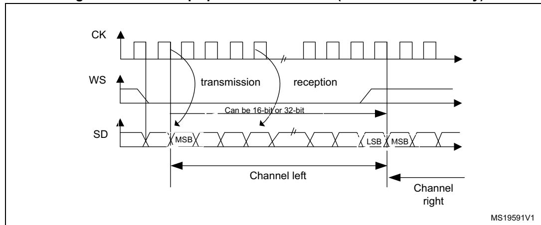
Figure 375. I 2 S Philips protocol waveforms (16/32-bit full accuracy)
