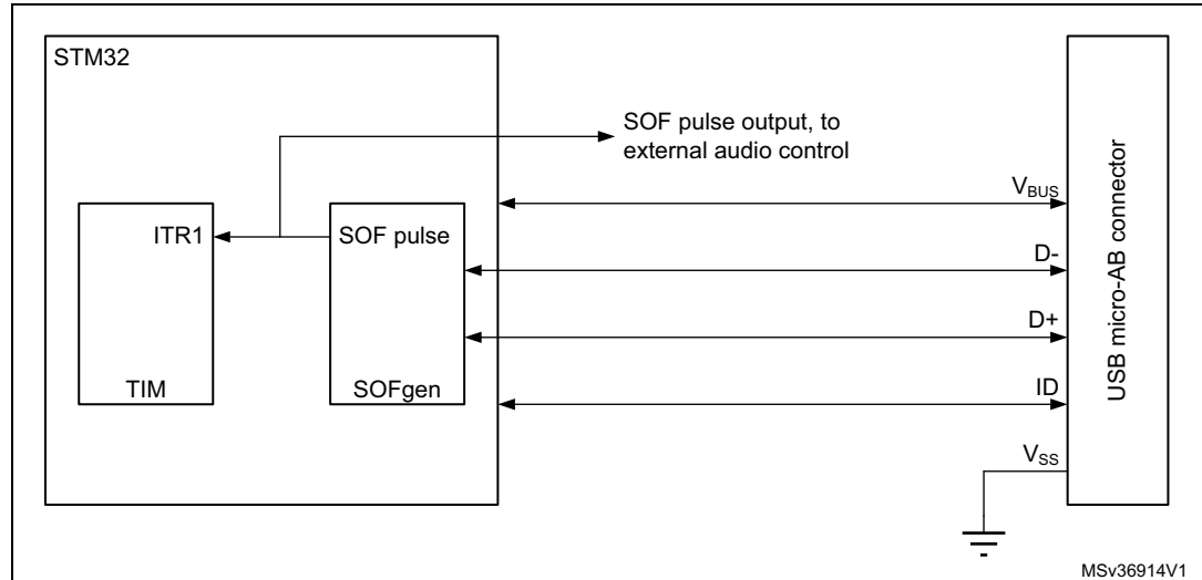
Figure 462. SOF connectivity (SOF trigger output to TIM and ITR1 connection)
