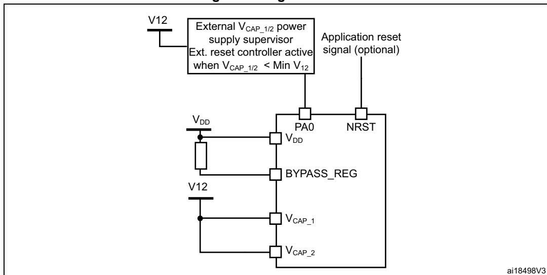
Figure 7. Regulator OFF
