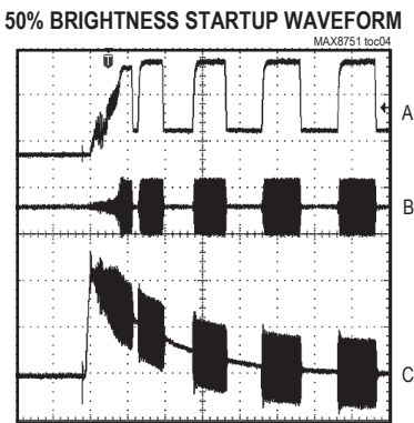
50% BRIGHTNESS STARTUP WAVEFORM MAX8751 toc04 A: COMP, 500mV/div B: IFB, 2V/div C: VFB, 1V/div
