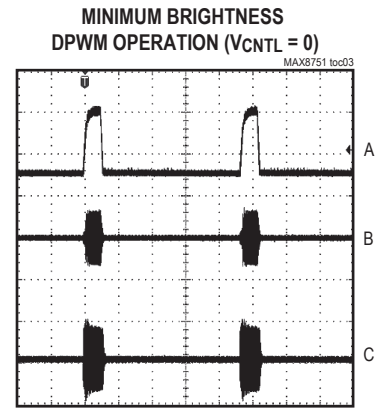
MINIMUM BRIGHTNESS DPWM OPERATION (VcNTL = 0) MAX8751 toc03 A: COMP, 500mV/div B: IFB, 2V/div C: VFB, 1V/div
