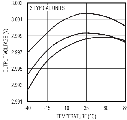
OUTPUT VOLTAGE vs. TEMPERATURE ( V_{OUT} = 3V )
