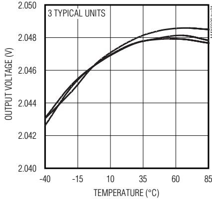
OUTPUT VOLTAGE vs. TEMPERATURE ( V_{OUT} = 2.048V )
