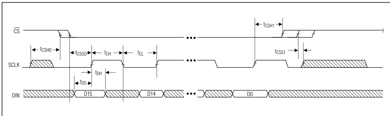
Figure 1. Timing Diagram
