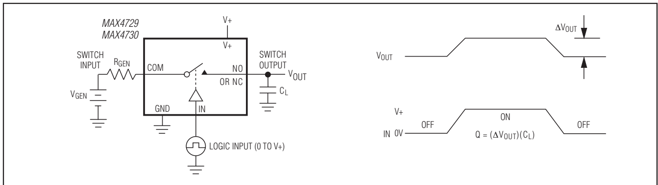
Figure 3. Charge Injection
