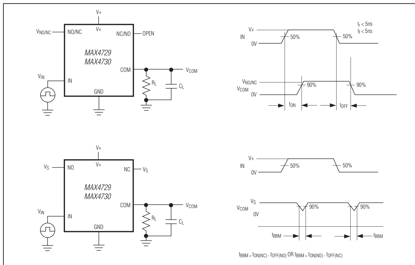
Figure 1. Switching Times
