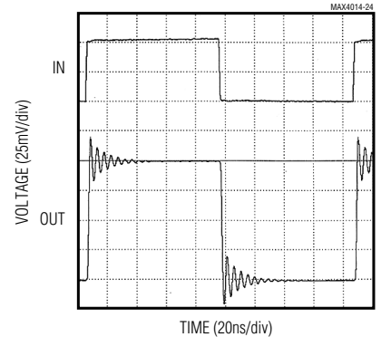
SMALL-SIGNAL PULSE RESPONSE (CL = 5pF)
