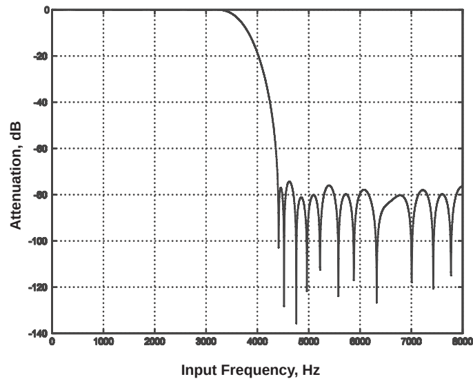
Figure 3-49. FIR Transmit Filter Response
