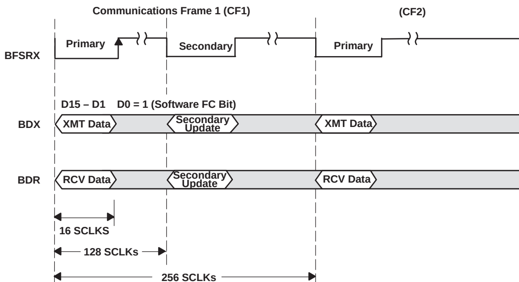
Figure 3–44. Software FC/ \overline{R/\overline{W}} DT Secondary Request
