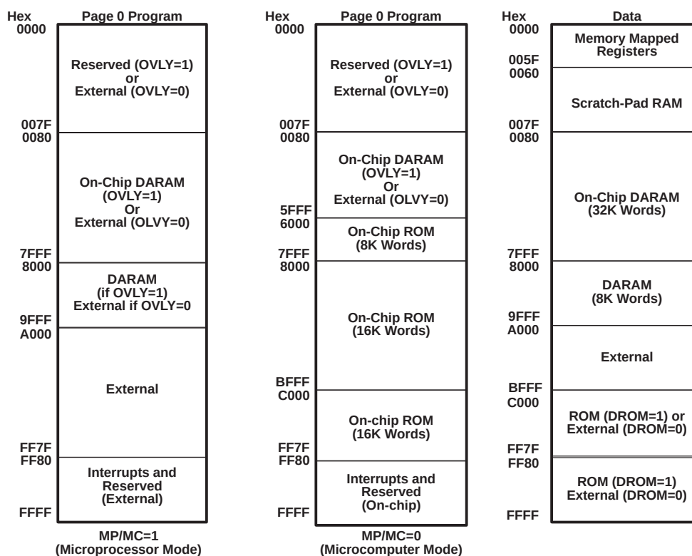
Figure 3-2. Program and Data Memory Map
