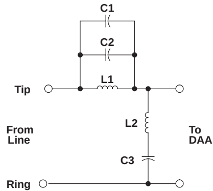
Figure 3-58. Billing Tone Filter
