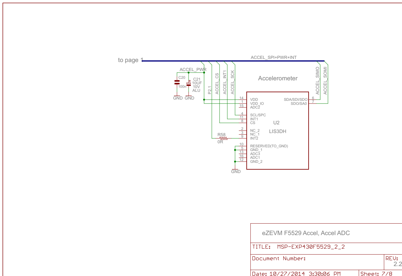
Figure 16. Schematics (7 of 8)
