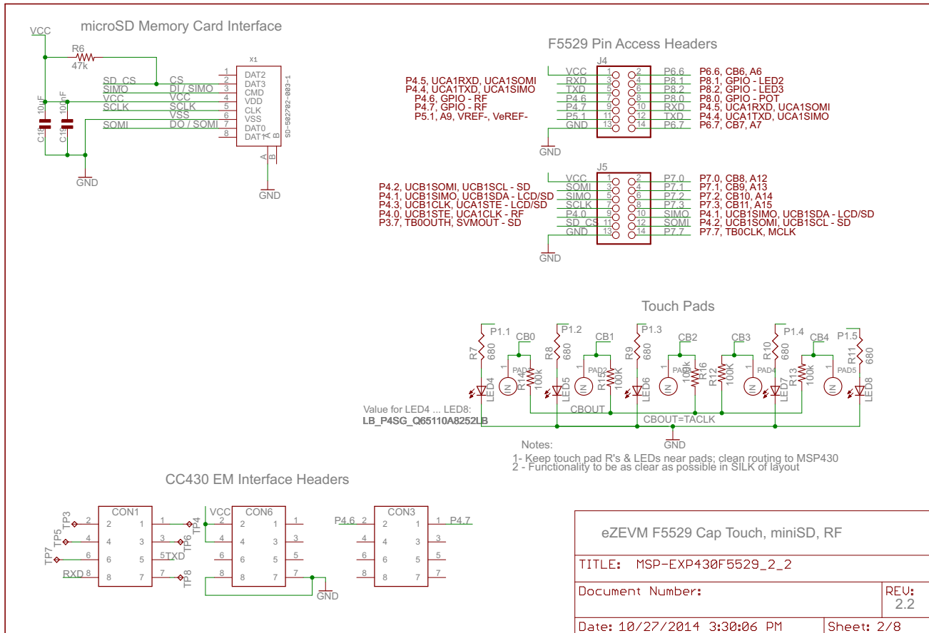
Figure 11. Schematics (2 of 8)
