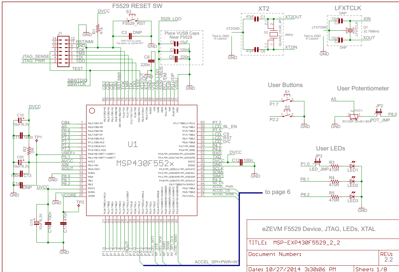
Figure 10. Schematics (1 of 8)
