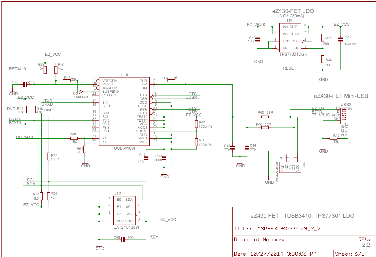
Figure 15. Schematics (6 of 8)
