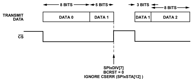
Figure 28. SPI Communication: Midbyte Stall
