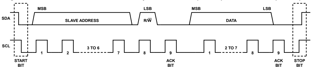
Figure 23. Typical I 2 C Transfer Sequence
