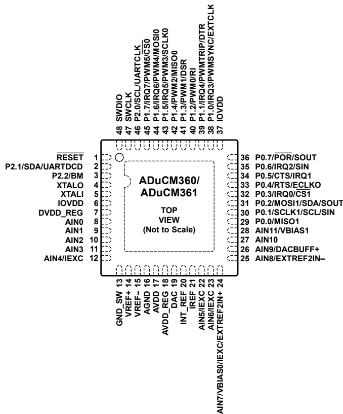
Figure 38. Pin Configuration
