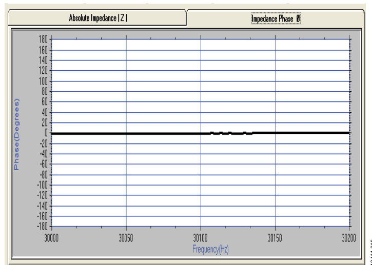
Figure 17. The Phase Tab on the AD5933 Evaluation Software Front Panel, Phase of 200 k \Omega Resistor (0°) Displayed
