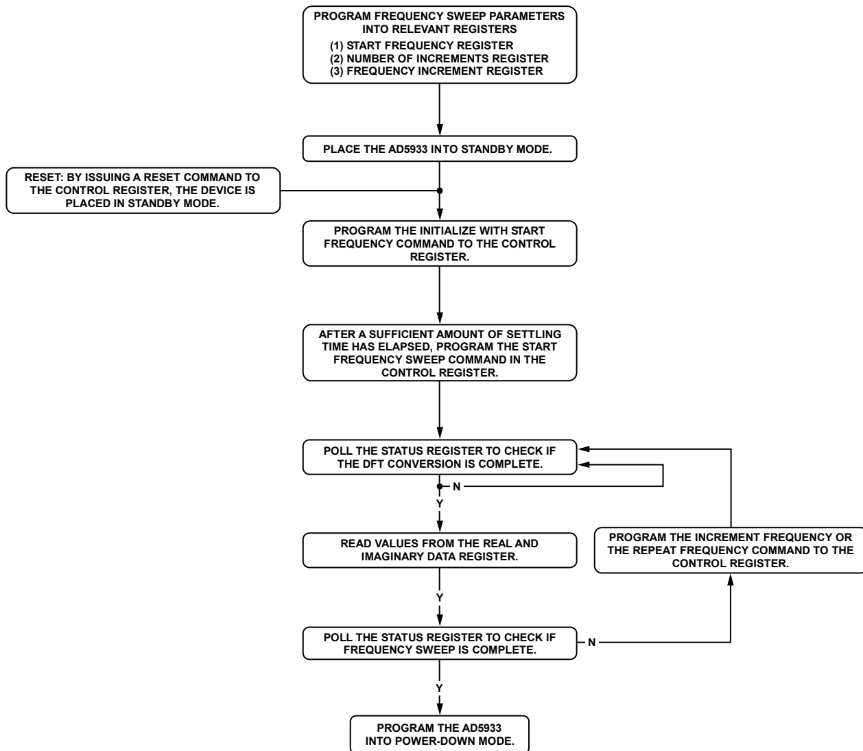
Figure 24. Sweep Flow Outline
