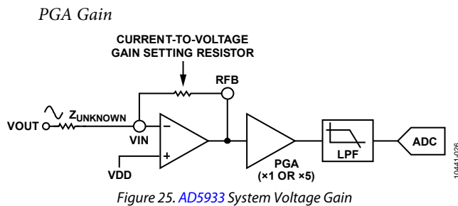
Figure 25. AD5933 System Voltage Gain
