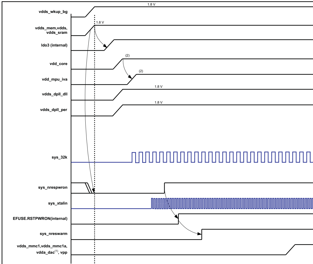
Figure 3-3. Power-up Sequence
