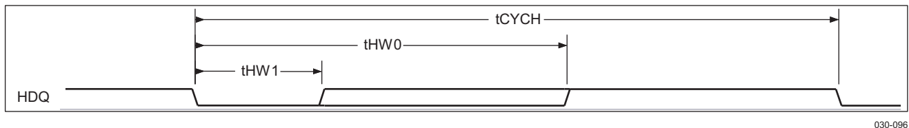
Figure 6-56. HDQ Read Bit Timing (Data)
