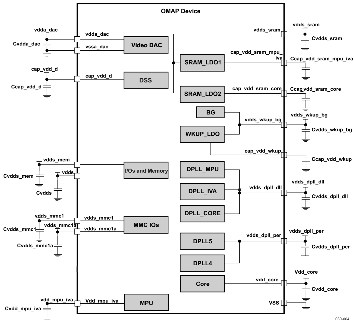
Figure 3-2. Power Supply Decoupling
