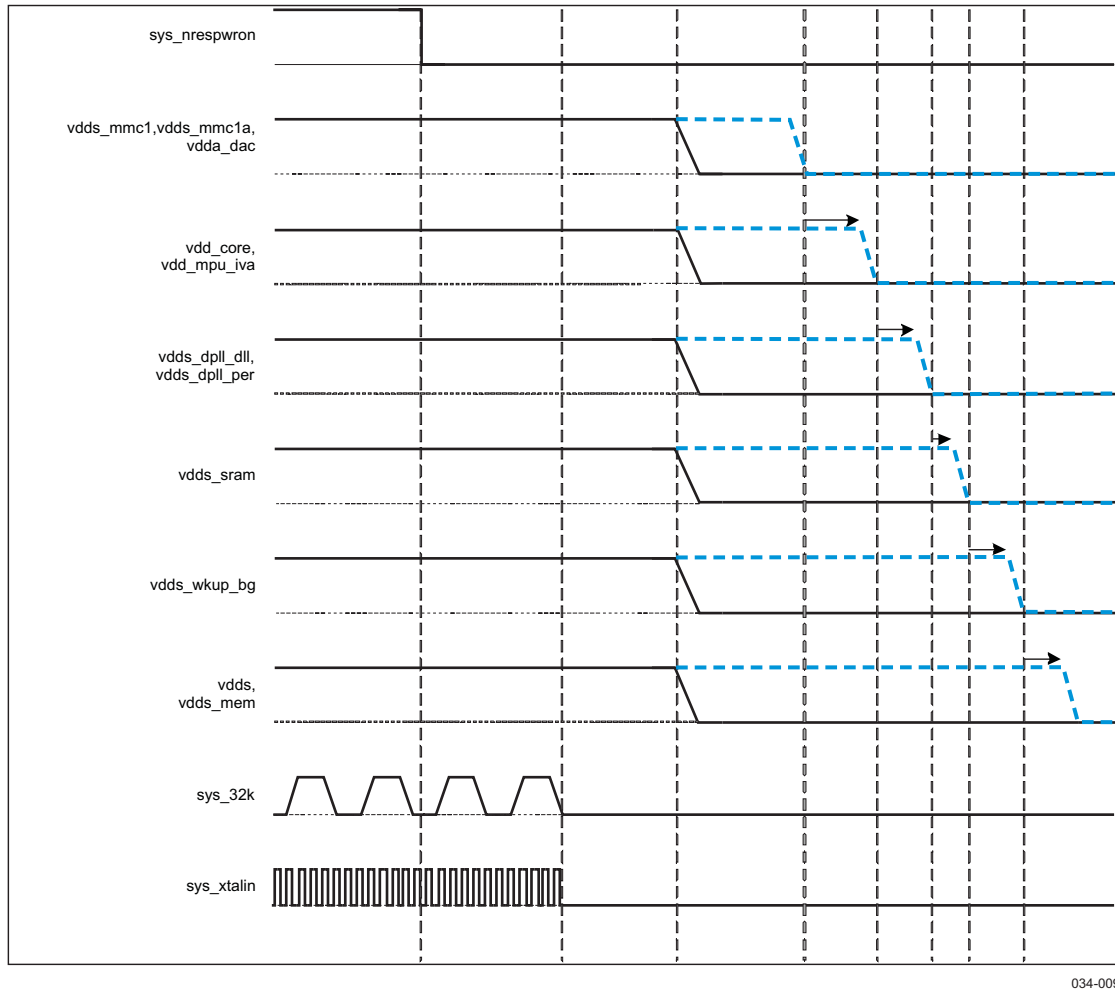
Figure 3-4. Power-down Sequence
