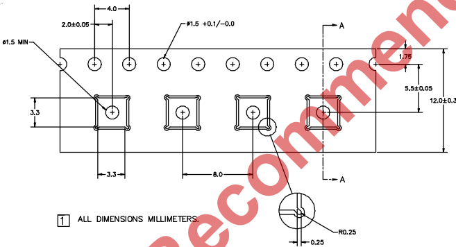
Tape Specifications
