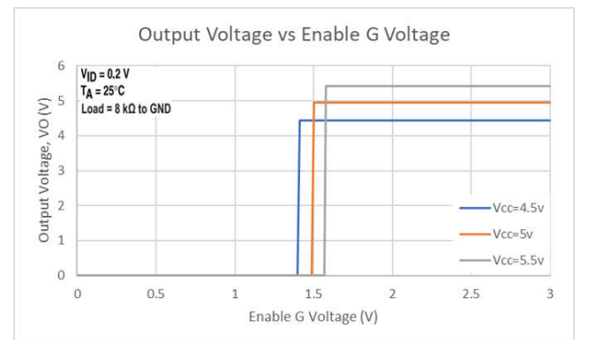
Figure 6-4. Output Voltage vs Enable G Voltage
