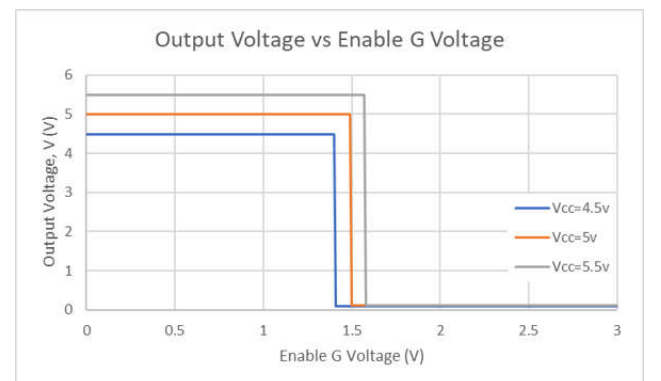
Figure 6-6. Output Voltage vs Enable G Voltage
