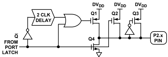
Figure 69. Internal Pull-Up Configuration
