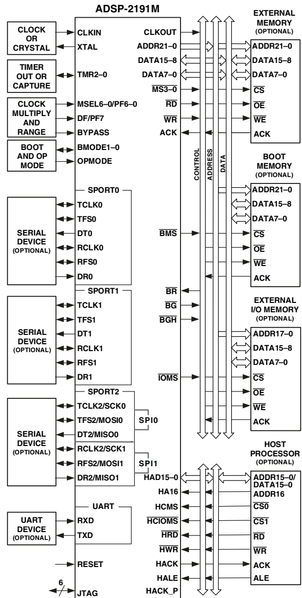
Figure 1. System Diagram
