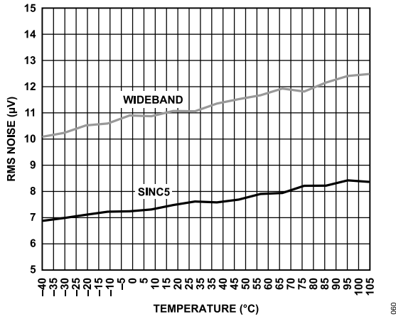
Figure 31. RMS Noise vs. Temperature, Low Power Mode
