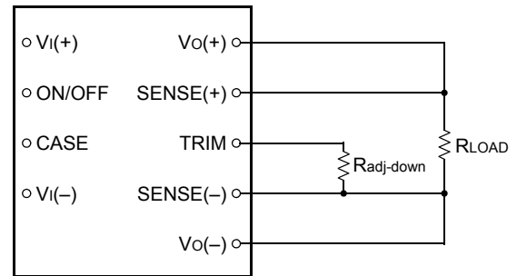
Figure 36. Circuit Configuration to Decrease Output Voltage.
