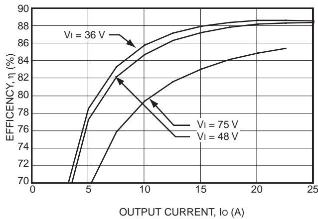
Figure 14. Converter Efficiency vs. Output Current.
