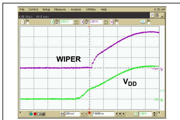
FIGURE 2-14: 2.1 kΩ – Power-Up Wiper Response Time.
