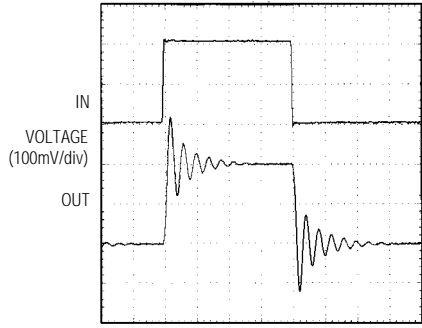
SMALL-SIGNAL PULSE RESPONSE ( A_{vCL} = +1V/V , C_L = 100pF )
