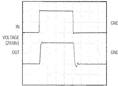
LARGE-SIGNAL PULSE RESPONSE ( A_{vCL} = +1V/V , C_L = 50pF )
