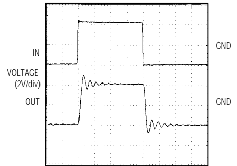
LARGE-SIGNAL PULSE RESPONSE ( A_{vCL} = +1V/V , C_L = 100pF )
