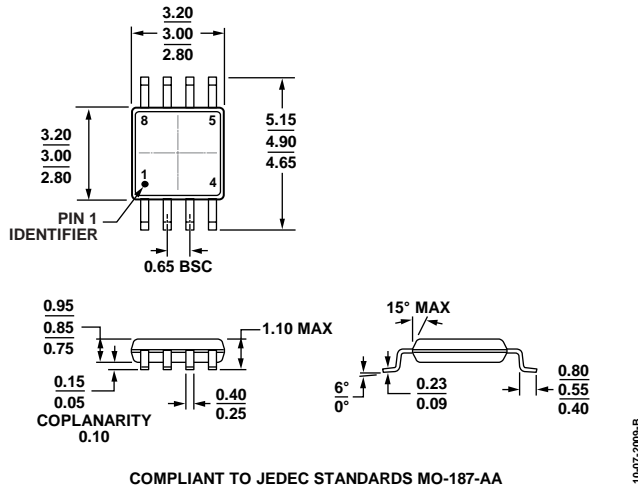
COMPLIANT TO JEDEC STANDARDS MO-187-AA Figure 107. 8-Lead Mini Small Outline Package [MSOP] (RM-8) Dimensions shown in millimeters
