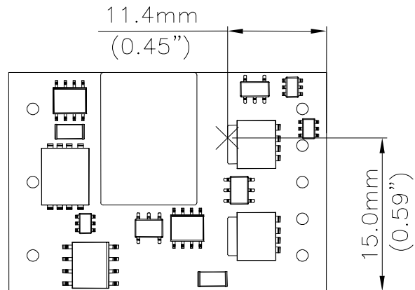
Figure 21: Temperature measurement location The allowed maximum hot spot temperature is defined at 127 .
