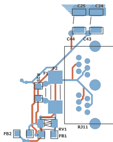
Figure 17. RJ11
