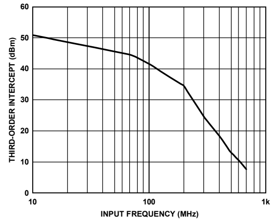
Figure 54. ADV3227 Third-Order Intercept, 100 Ω Load
