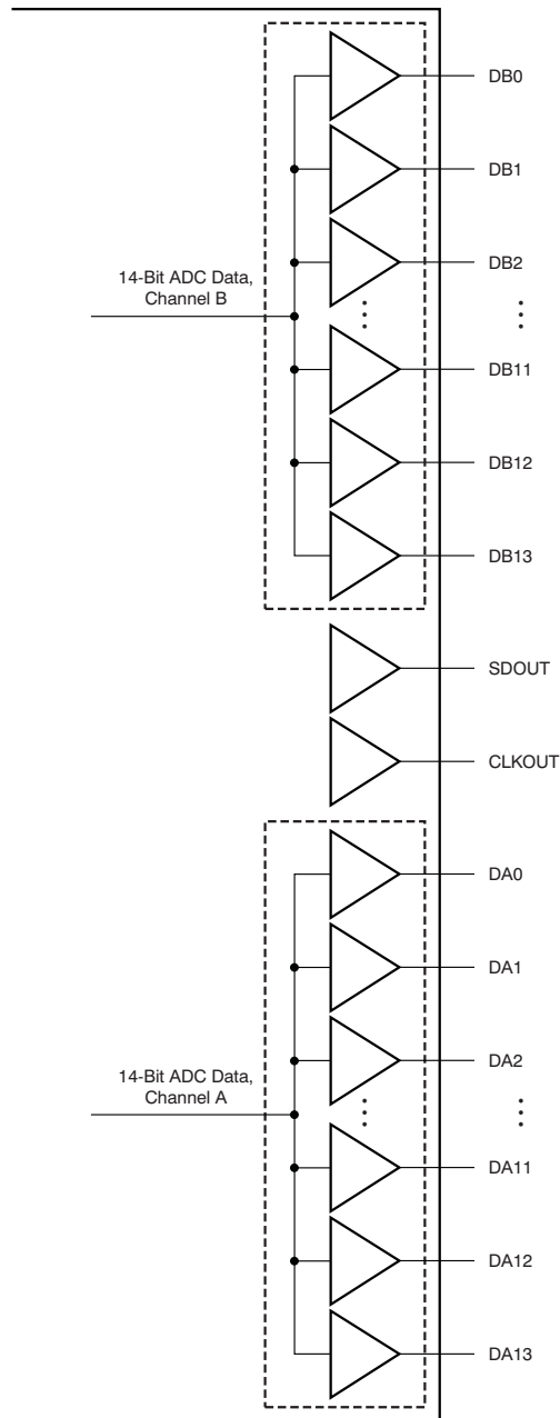
Figure 158. CMOS Outputs
