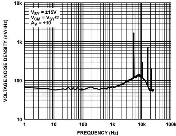
Figure 50. Voltage Noise Density vs. Frequency
