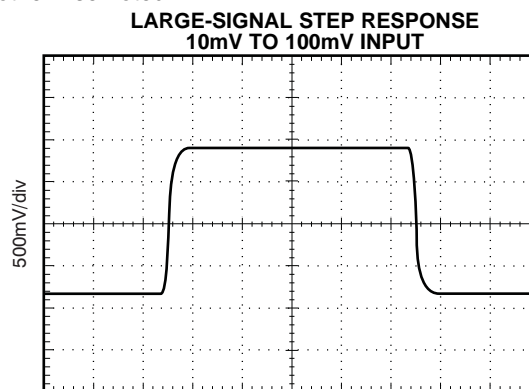
10µs/div Figure 15.
