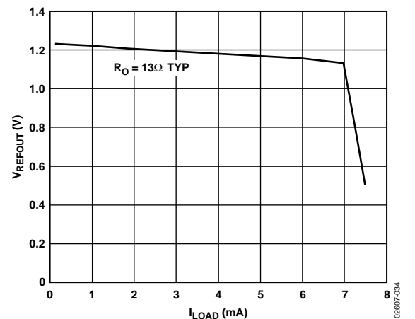
Figure 34. V_{REFOUT} vs. I_{LOAD}
