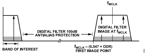
Figure 42. AD7766/AD7766-1/AD7766-2 Spectrum
