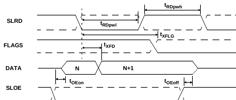
Figure 10-8. Slave FIFO Asynchronous Read Timing Diagram [17]
