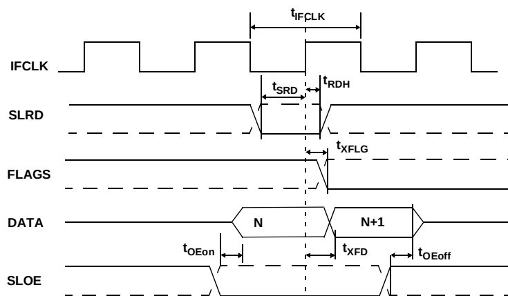
Figure 10-7. Slave FIFO Synchronous Read Timing Diagram [17]
