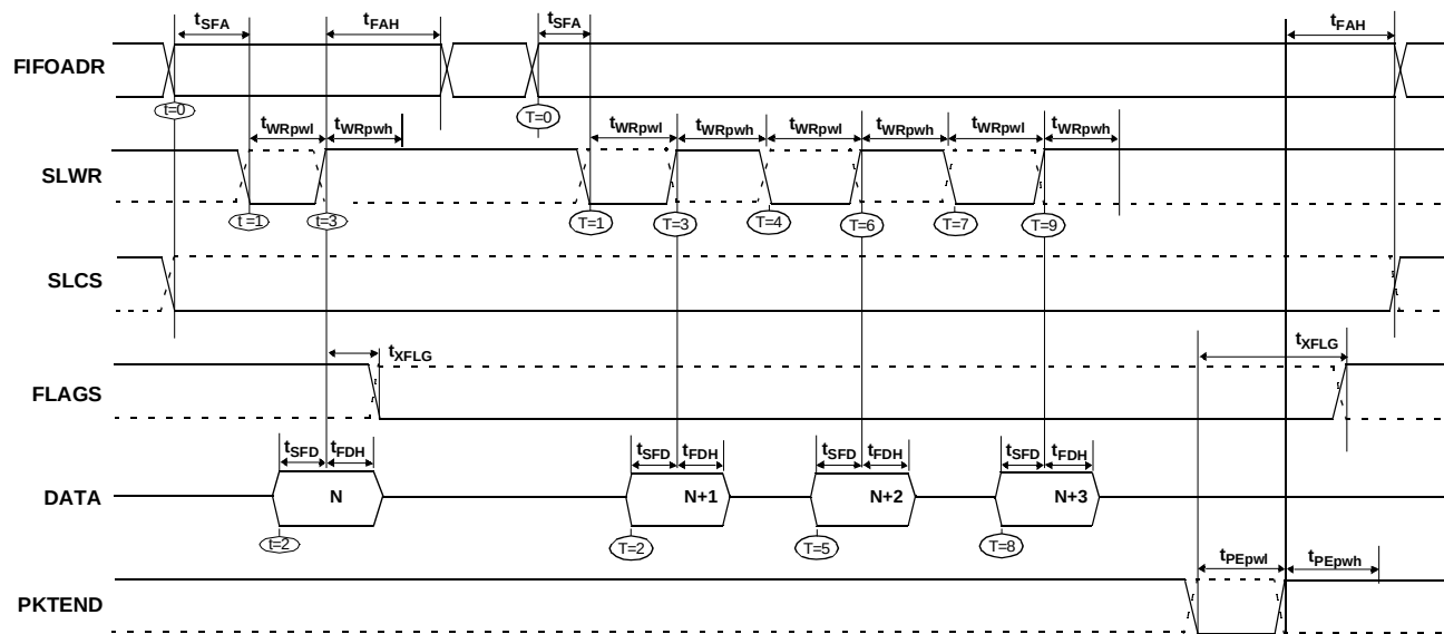
Figure 10-23. Slave FIFO Asynchronous Write Sequence and Timing Diagram [17]
