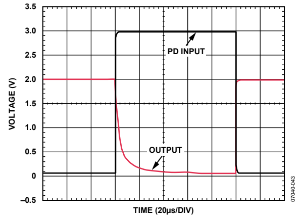
Figure 42. Disable/Enable Switching Speed
