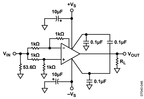
Figure 52. Common-Mode Rejection
