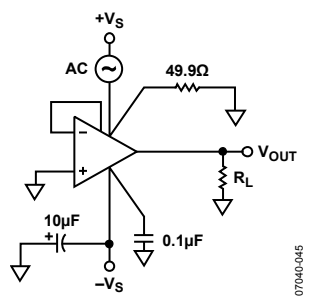
Figure 50. Positive Power Supply Rejection
