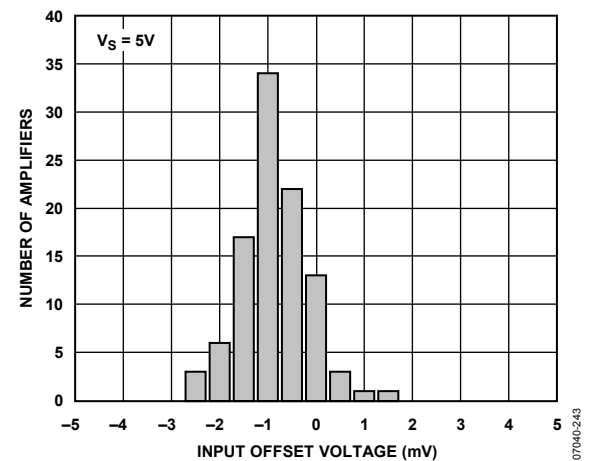
Figure 43. Input Offset Voltage Distribution, V_S = 5 V
