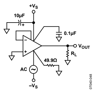
Figure 53. Negative Power Supply Rejection
