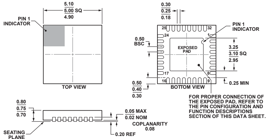
COMPLIANT TO JEDEC STANDARDS MO-220-WHHD. Figure 12. 32-Lead Lead Frame Chip Scale Package [LFCSP_WQ] 5 mm x 5 mm Body, Very Very Thin Quad (CP-32-7) Dimensions shown in millimeters
