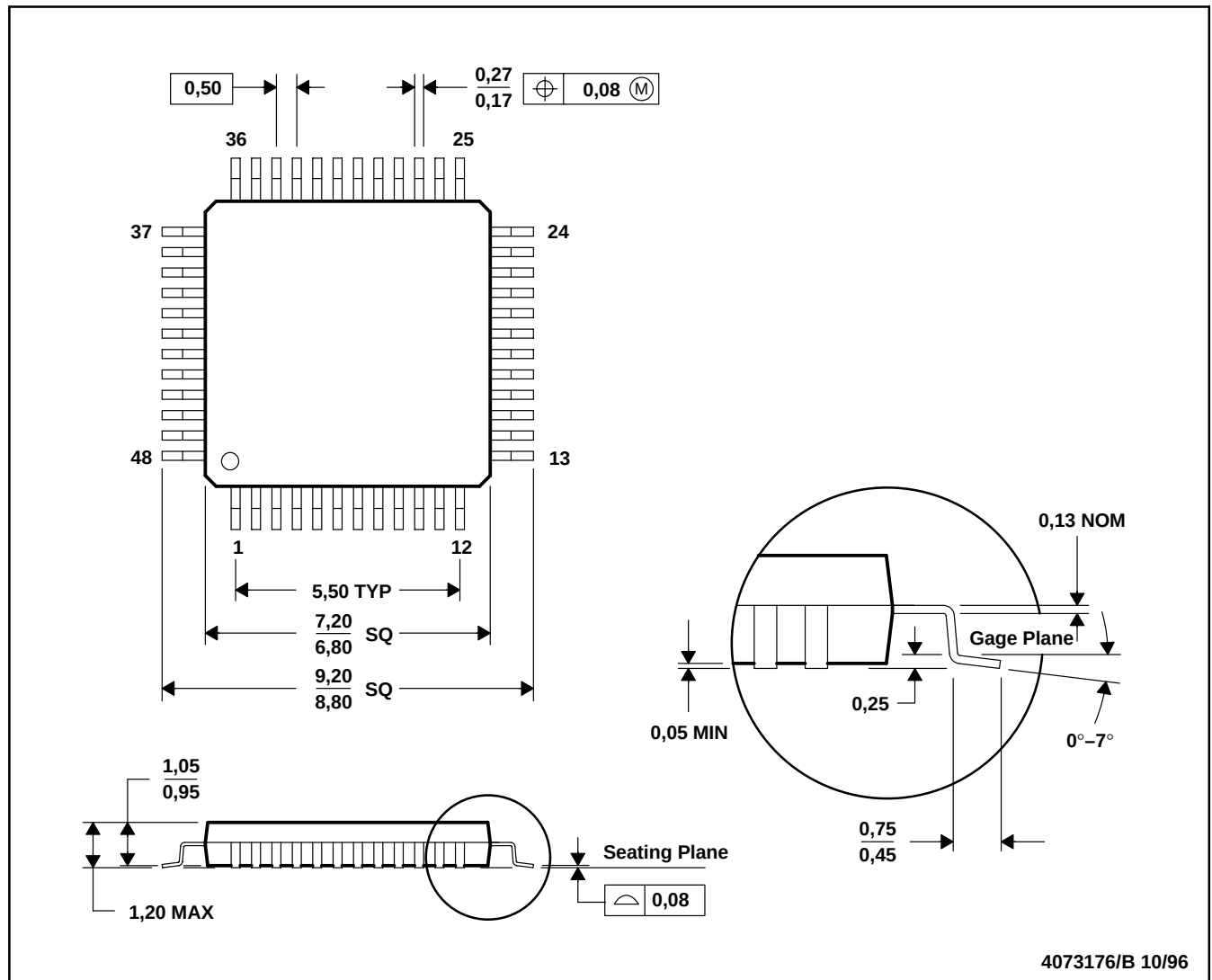
PFB (S-PQFP-G48)
