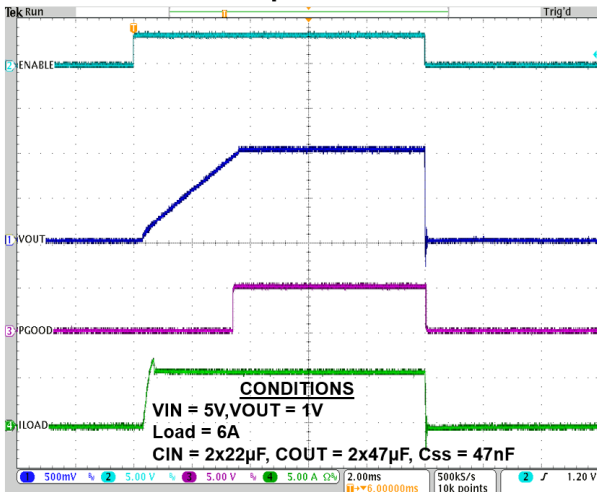
Startup Waveform
