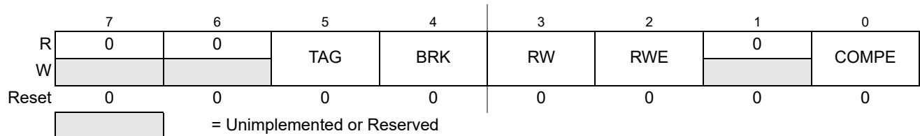
Figure 8-15. Debug Comparator Control Register DBGCCCTL (Comparator C)
