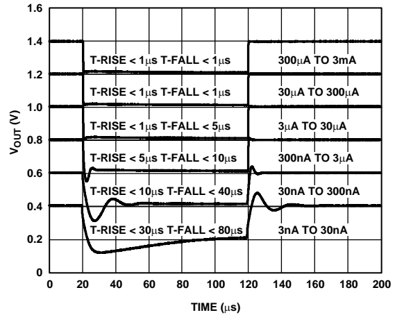
Figure 18. Pulse Response— I_{INP} to V_{OUT} ( A_V = 1 ) in Consecutive 1-Decade Steps
