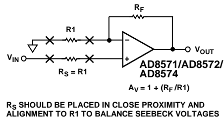
Figure 55. Using Dummy Components to Cancel Thermoelectric Voltage Errors
