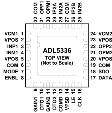
Figure 4. Pin Configuration
