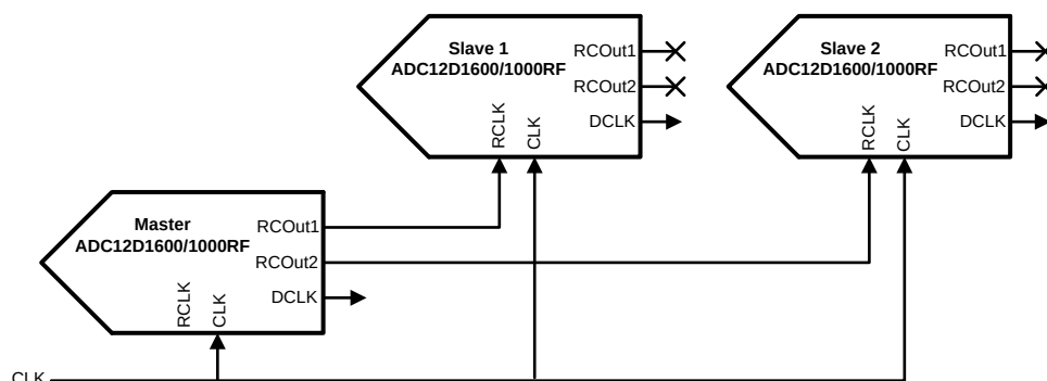
Figure 6-5. AutoSync Example
