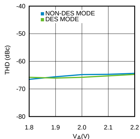
Figure 4-26. THD vs Supply Voltage (ADC12D1600RF)
