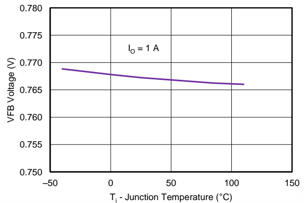
Figure 12. VFB VOLTAGE vs JUNCTION TEMPERATURE (IO = 1 A)
