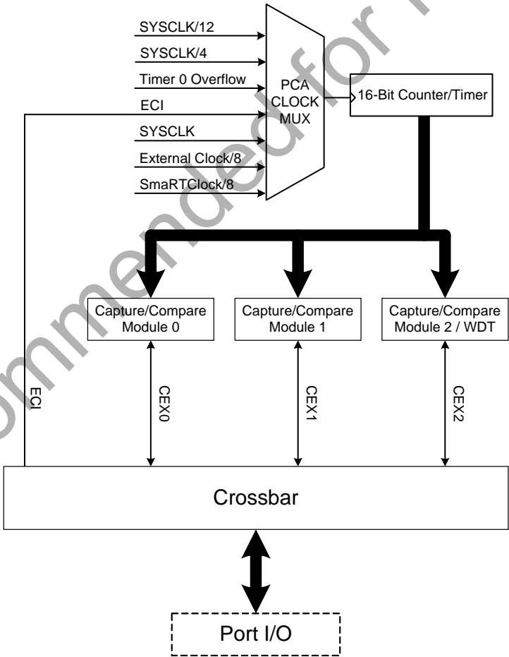
Figure 26.1. PCA Block Diagram
