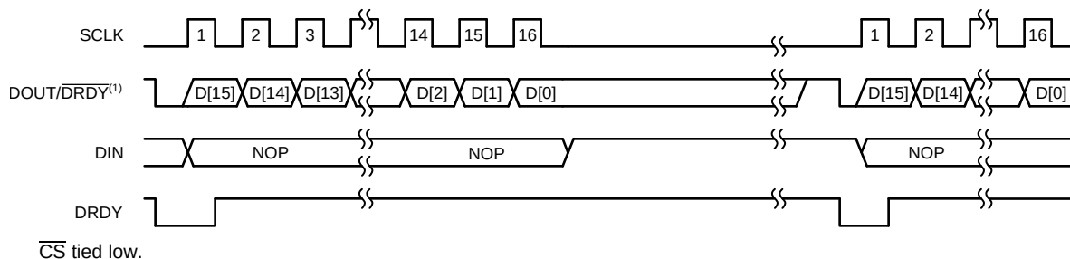
Figure 42. Data Retrieval With the DRDY MODE Bit = 1 (Enabled)
