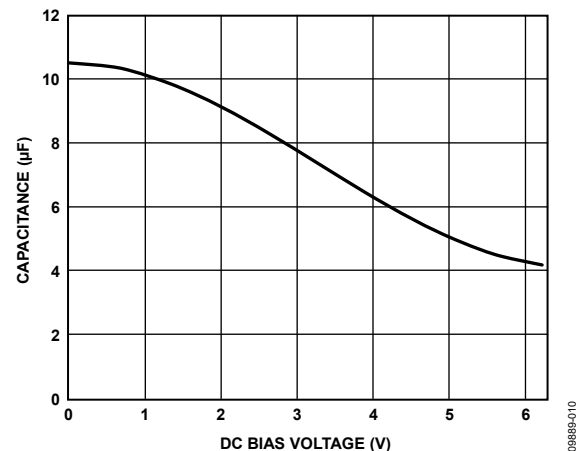
Figure 49. Capacitance vs. Voltage Characteristic
